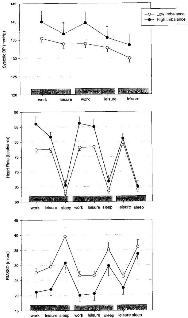
Figure 2. SBP, HR, and RMSSD (mean±SD) during work, leisure, and sleep (only HR and RMSSD) on 2 workdays and 1 nonworkday for the high- (●) and low-imbalance (○) groups.
