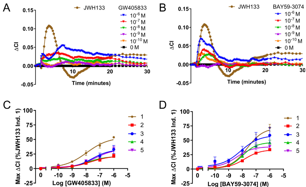
Fig. 6. Individual CB 2 R responses from two partial agonists. Cell lines were stimulated with agonist 18 h after seeding (100,000 cells/well, fibronectin 50 μg/ml). Representative graph of the baseline-corrected response to (A) GW405833 and (B) BAY59-3074 [1 μM – 100 pM] from individual 1. Resulting concentration-effect curves of (C) GW405833 and (D) BAY59-3074 obtained from peak ΔCI normalized to JWH133 [1 μM] effect on individual 1. Data represent mean ± SEM obtained from three independent experiments performed in duplicate.
