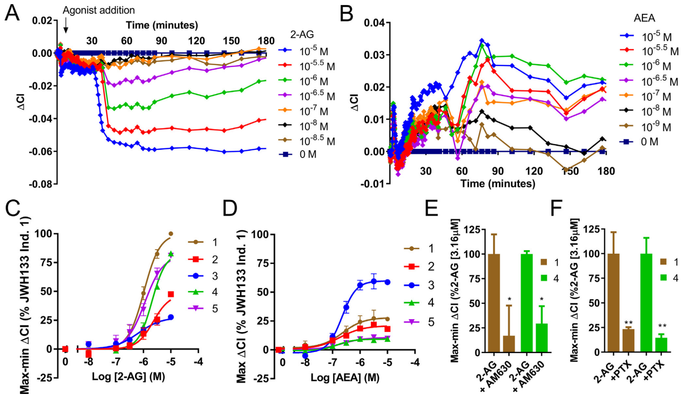
Fig. 5. Individual CB 2 R responses to endocannabinoids. Cell lines were stimulated with 2-AG (50,000 cells/well, fibronectin 10 μg/ml) or AEA (100,000 cells/well, fibronectin 50 μg/ml) 18 h after seeding. Representative graphs of the baseline-corrected (A) 2-AG [10 μM – 3.16 nM] and (B) AEA [10 μM – 1 nM] response from individual 1. (C) Concentration-effect curves of 2-AG were obtained from Max-Min ΔCI within 1 h of stimulation were normalized to E max of CB 2 R-selective agonist JWH133 response on individual 1. (D) Concentration-effect curves of AEA were obtained from Max ΔCI normalized to E max of CB 2 R-selective agonist JWH133 response on individual 1. Next, bar graphs show the inhibition of the 2-AG effect by (E) CB 2 R-selective antagonist AM630 [10 μM] and (F) Gα i -inhibitor PTX normalized to 2-AG's effect at EC 50 (3.16 μM). Data represent the means ± SEM from three or four (C, D) or means ± SD of two (E, F) independent experiments performed in duplicate. Significance of inhibitor effect versus 2-AG response only was determined with a two-way ANOVA Fisher's LSD test * = p < 0.05, ** = p < 0.01. AM630 and PTX inhibition did not differ significantly between individuals 1 (R63) and 4 (Q63) as determined using a two-way ANOVA with a Sidak post-hoc test.
