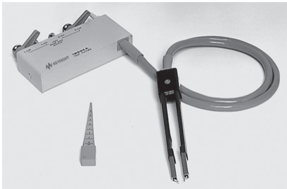
16334A SMD/chip tweezers test fixture
