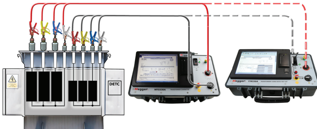
The diagram shows the MTO3XX series and TTR3XX series easily and conveniently using the same set of test leads. For example, the user can leave the leads connected to the transformer and use the same lead set to run turns-ratio testing with the Megger TTR3XX series, eliminating several up-and-down-the-ladder trips.
