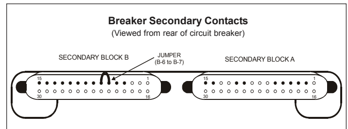
Figure 6. Breaker Secondary Contact Jumper for Ground Fault Test (Magnum or Medium Voltage Breaker).
