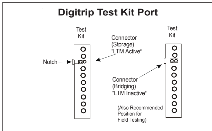
Figure 4. Long Time Memory (LTM) Jumper.
