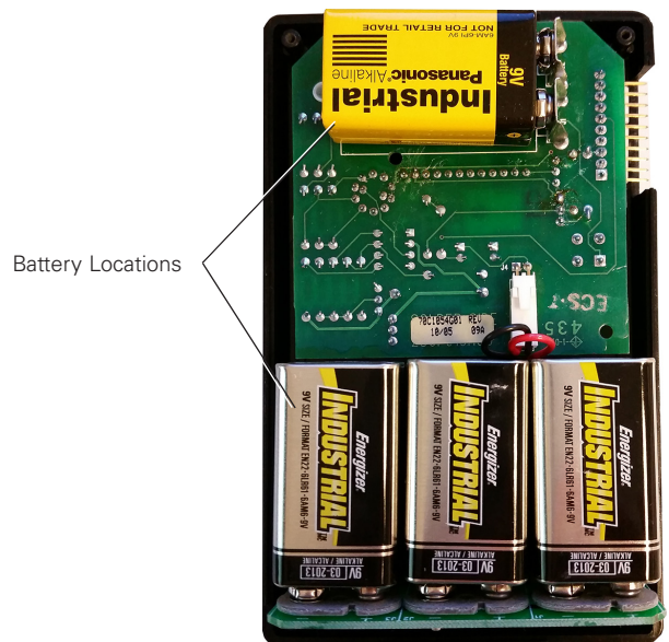
Figure 3. Battery Locations.
