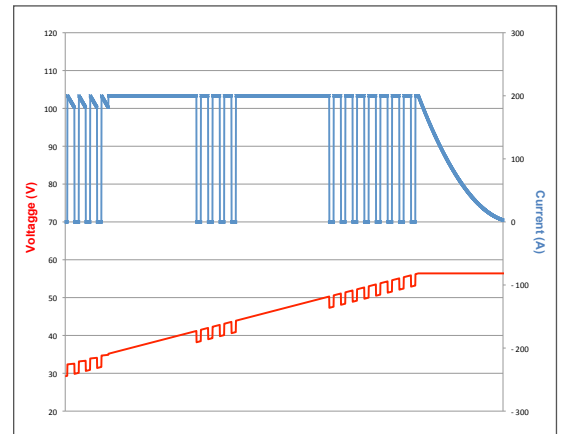
Figure 3 - Series Resistance In Use
