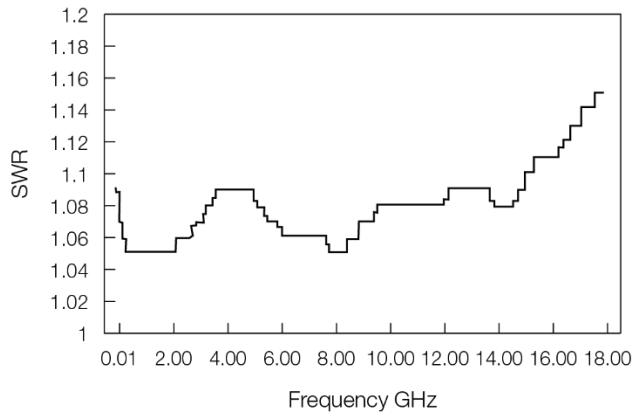
Typical SWR, 10 MHz to 18 GHz ( 25\text{ }^{\circ}\text{C} \pm 10\text{ }^{\circ}\text{C} ) for E9300A and E9301A sensor.
