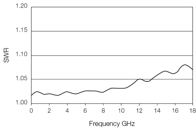
Typical SWR, 10 MHz to 18 GHz ( 25\text{ }^{\circ}\text{C} \pm 10\text{ }^{\circ}\text{C} ) for E9300B and E9301B sensors.
