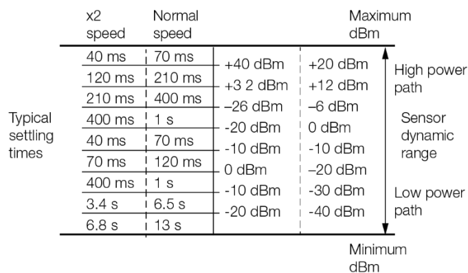
With E-Series E9300B/01B/00H/01H sensor
