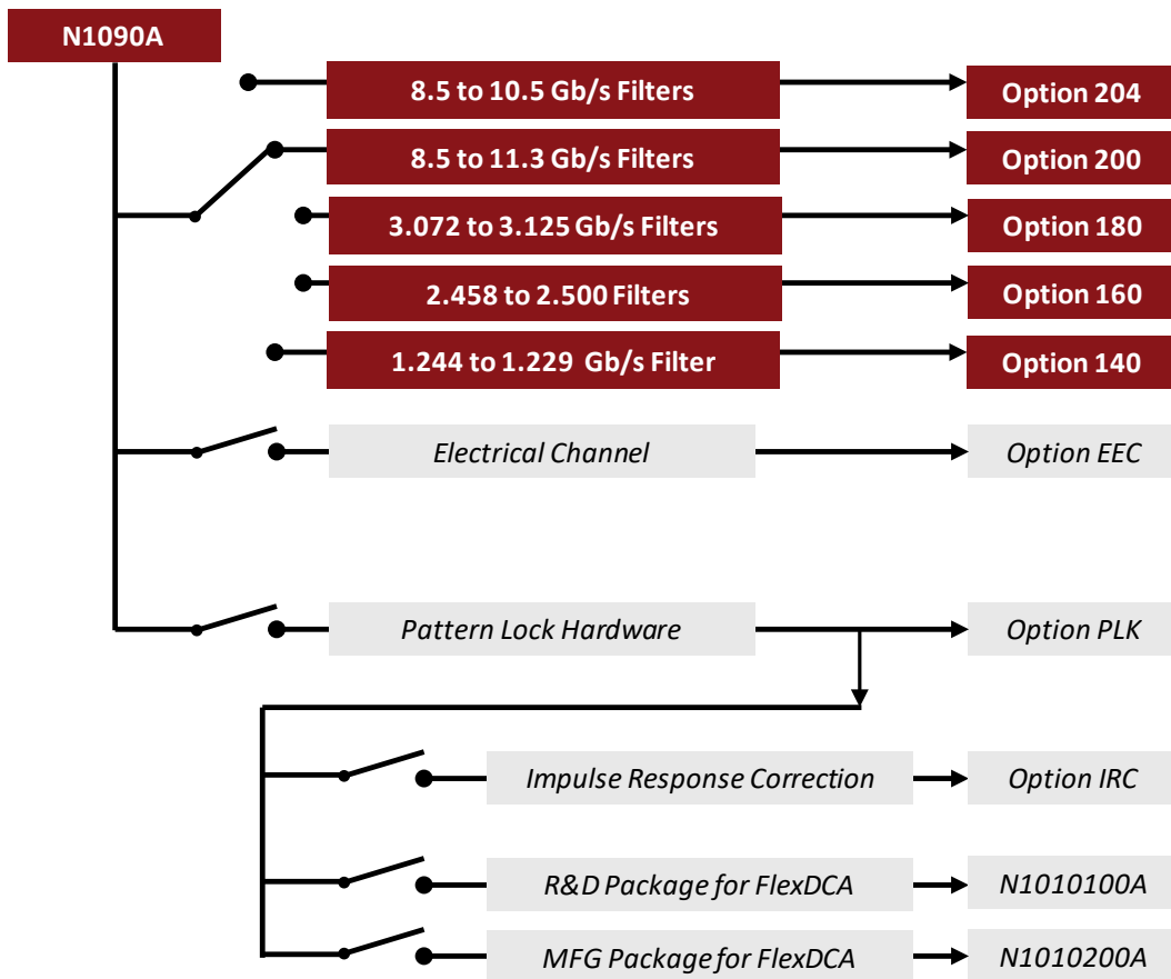
Figure 31: N1090A configuration chart
