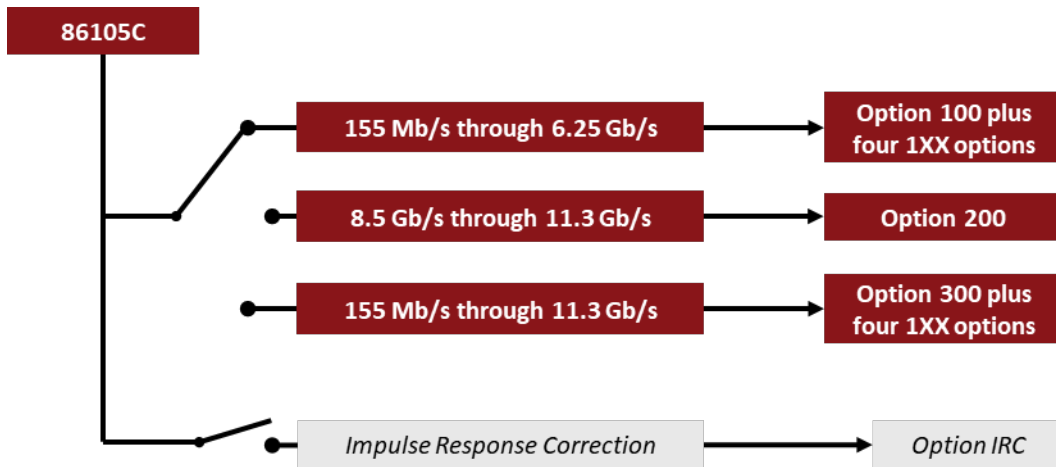
Figure 2: 86105C module with options 130, 150, 180, 190, 300
