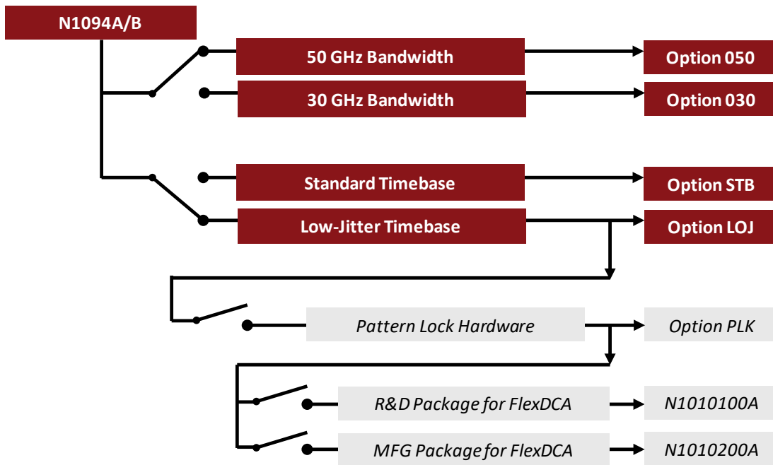
Figure 35: N1094A/B configuration chart
