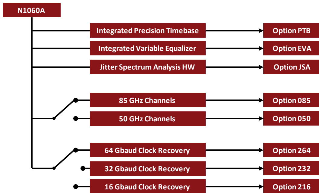
Figure 23: N1060A configuration chart
