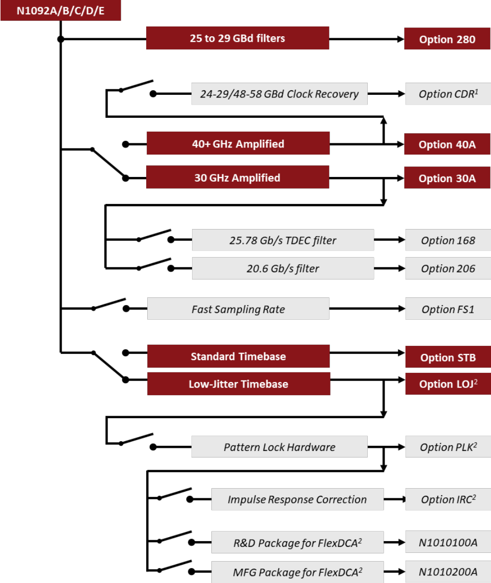
Figure 33: N1092A/B/C/D/E configuration chart
