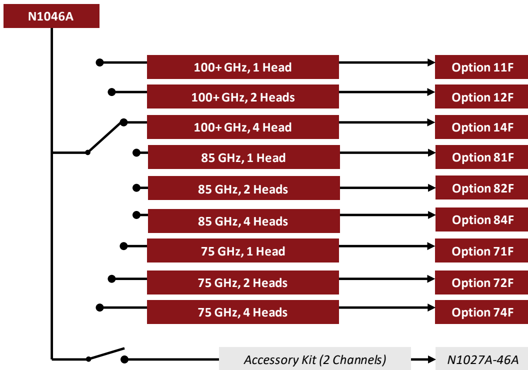
Figure 19: N1046A configuration chart
