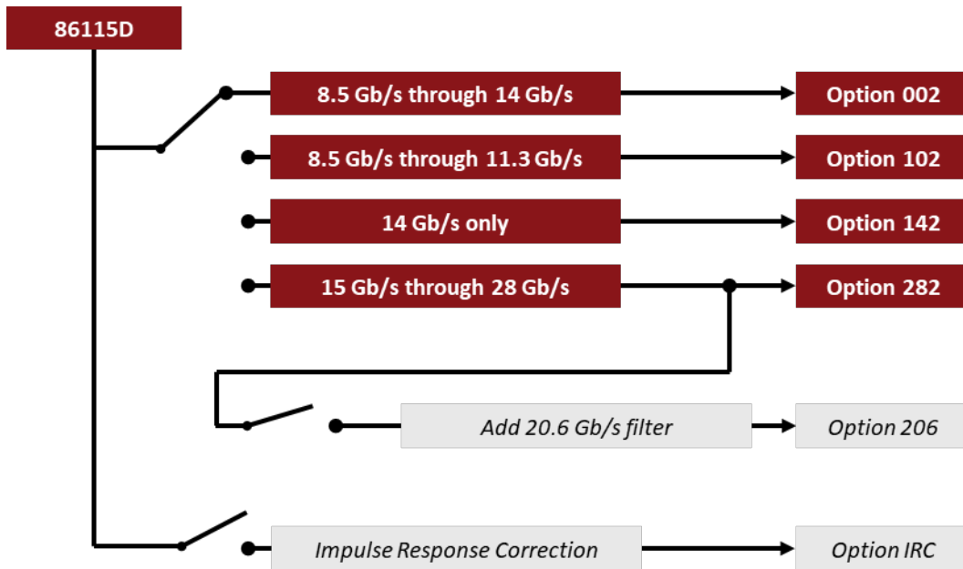
Figure 7: 86115D configuration chart
