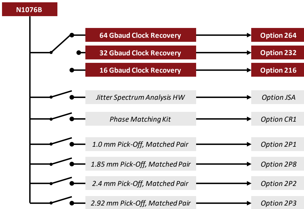
Figure 24: N1076B Electrical clock recovery with option 264
