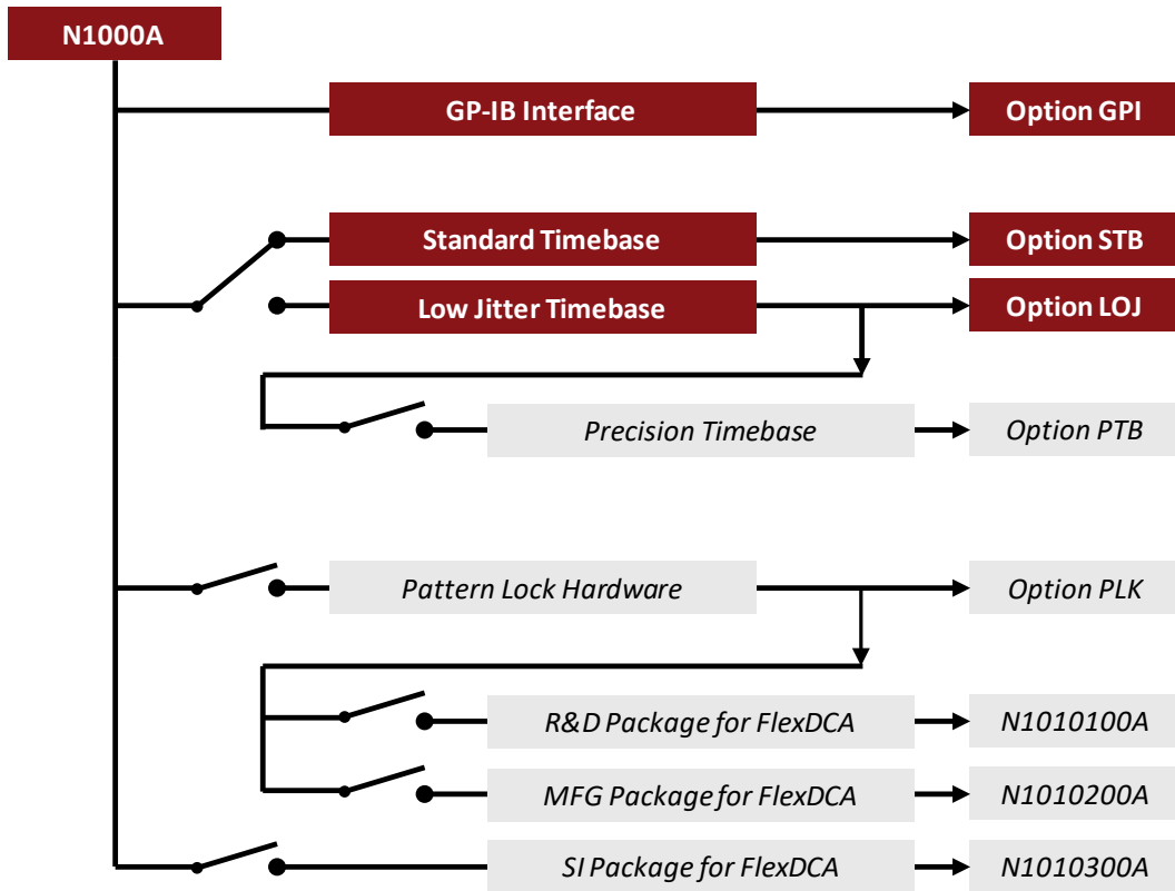
Figure 11: N1000A configuration chart
