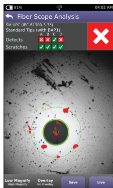
Fiber Scope Analysis
