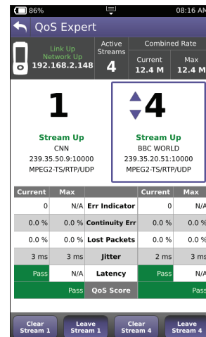
OneExpert DSL IP Video — QoS Expert
