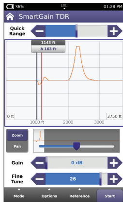
Standard TDR mode
