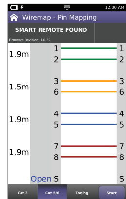
Wire mapping
