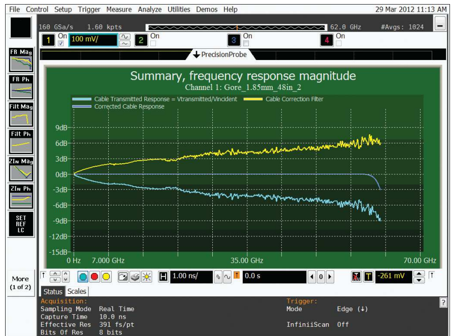
Figure 7. Example of frequency response correction of a cable. The 3dB down point moved from 21 GHz to 62 GHz.
