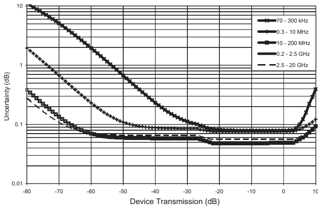
Transmission Magnitude Uncertainty (1 of 2) MS4647B with LRL Calibration using 3657-1 Cal Kit (> 5 GHz) with LRM Calibration using 3654D Cal Kit (< 5 GHz)
