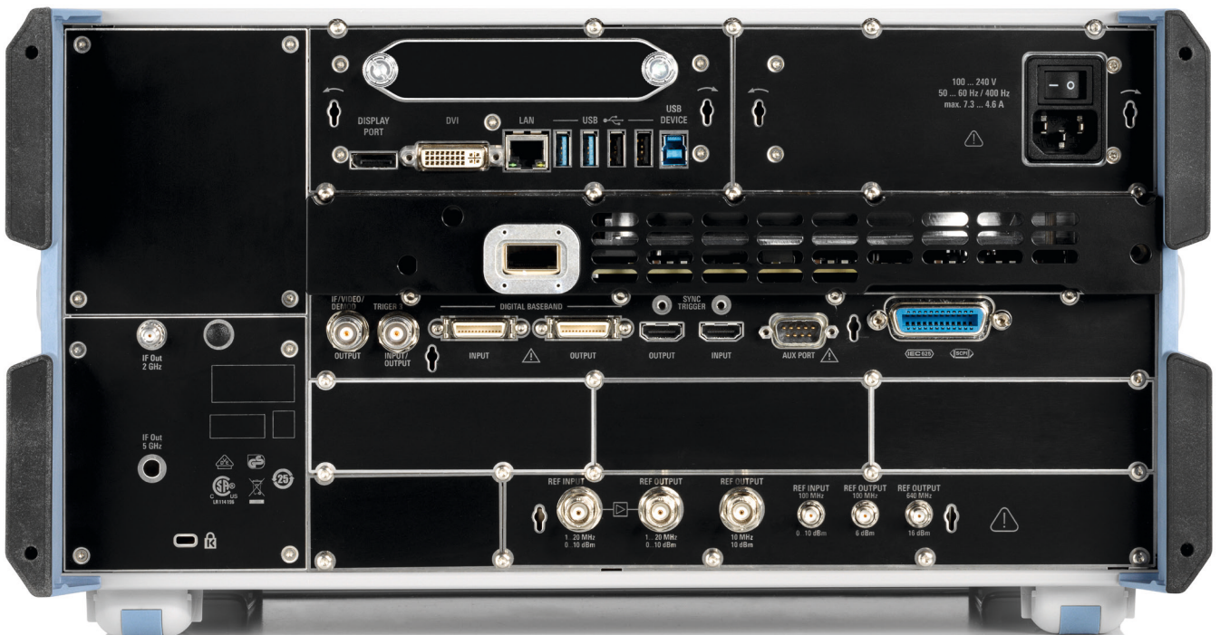
Rear view of the R&S®FSW
