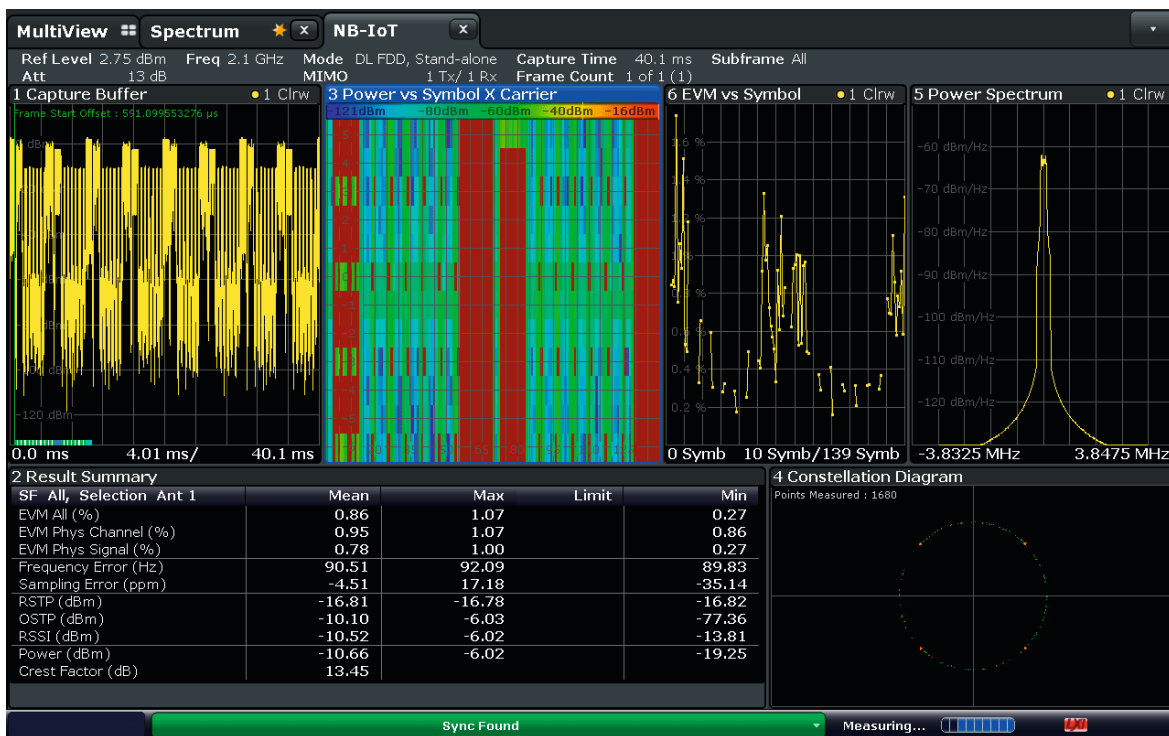
The R&S®FSW-K106 NB-IoT measurement application
