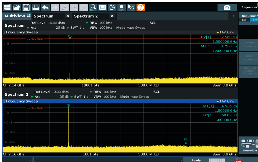
Harmonic measurement with highpass filter switched on (top) and off (bottom)
