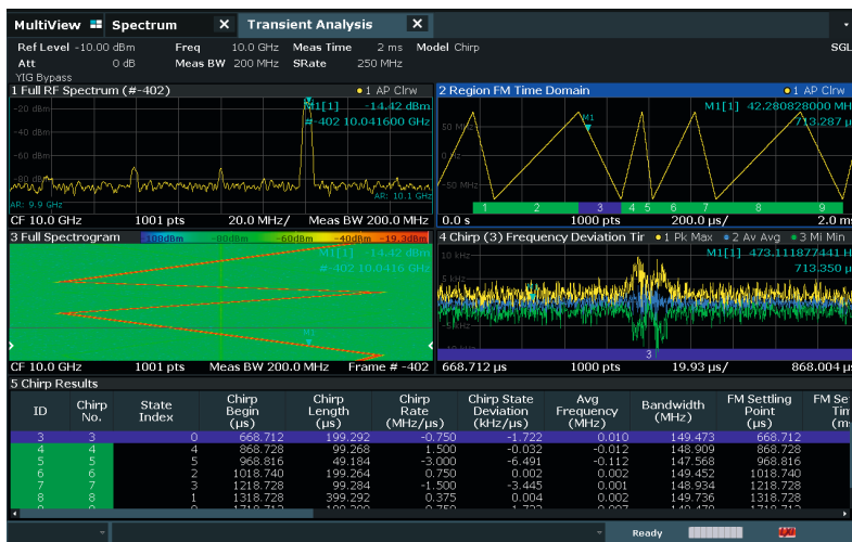
Analysis of an FMCW signal with the R&S®FSW-K60C option.
