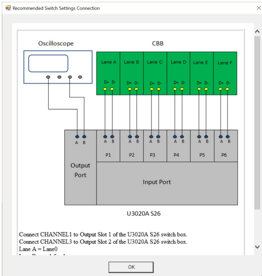
Figure 16a. A connection diagram is provided to help setup the switch
