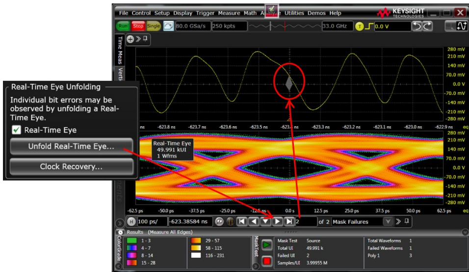
Figure 20. Once the mask test is complete the Serial Data Analysis application allows you to show the specific signal within the waveform that caused failures
