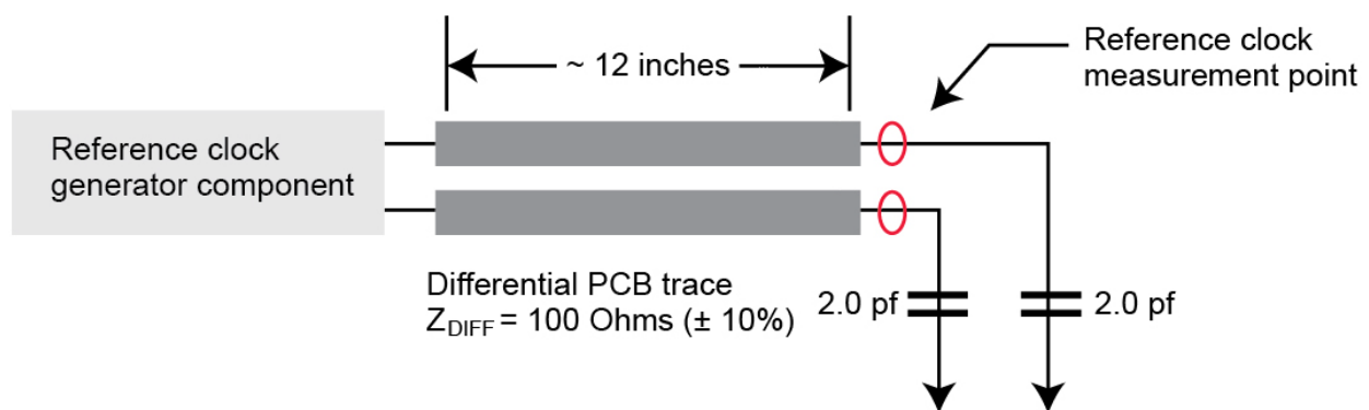
Figure 17. This figure shows the reference clock compliance channel, compliance load, and probing requirement for all PCIe 4.0 reference clock tests. Note that these tests are intended to be used to validate your PCIe reference clock at the component level
