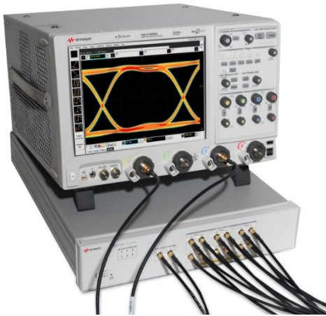
Figure 15. Automated testing for multi-lane digital bus interface through switching solution
