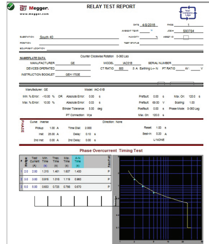
Figure 5: Test report G.E. IAC 51B inverse timing test
