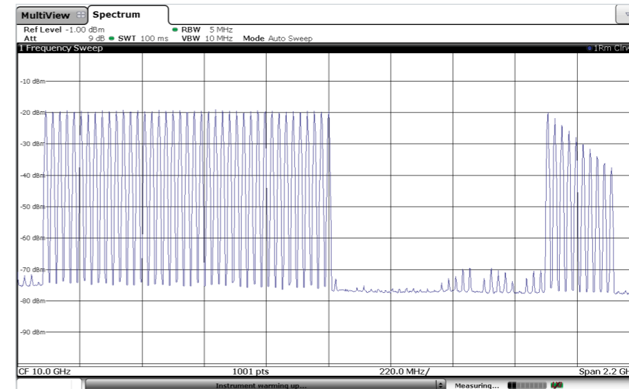
The R&S®SMW200A generates top-quality wideband signals, including signals that are asymmetrical to the center frequency. In this example, at 10 GHz a 2 GHz wide multicarrier CW scenario with 41 equal-power carriers is generated on the left and 10 carriers with graduated power on the right.
