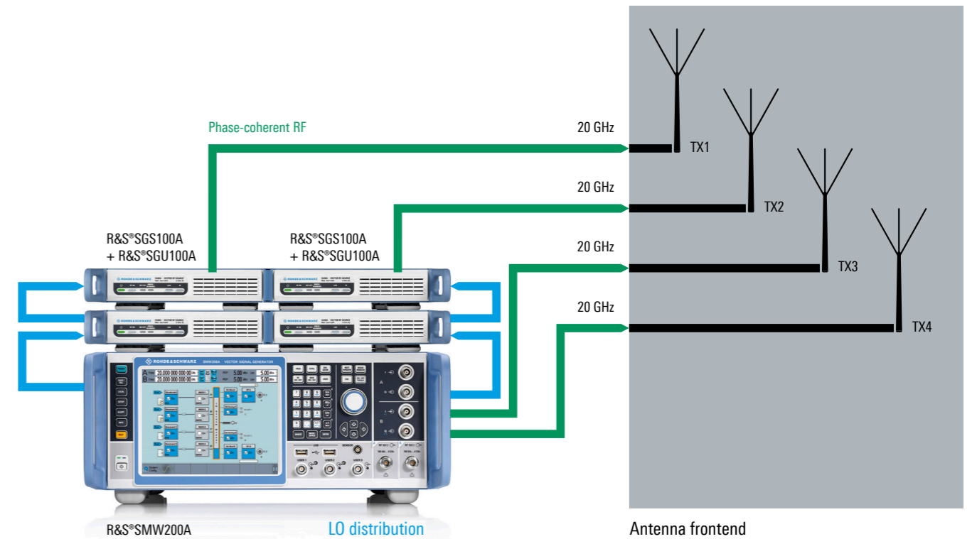
Setup with a two-path R&S®SMW200A, two R&S®SGS100A and two R&S®SGU100A to generate four phase-coherent CW or modulated signals, for example for antenna testing up to 20 GHz. The setup can be scaled to 40 GHz and duplicated if more RF paths are required.
