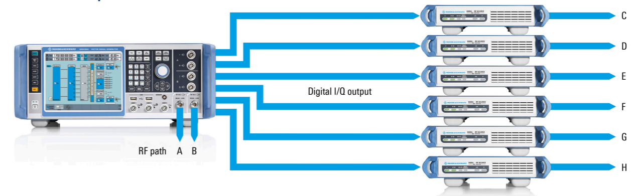
4x8 MIMO setup, consisting of a two-path R&S®SMW200A and six R&S®SGT100A signal generator modules operated from the R&S®SMW200A. The modules provide RF paths 3 to 8. The R&S®SMW200A fully performs baseband signal generation and fading.
