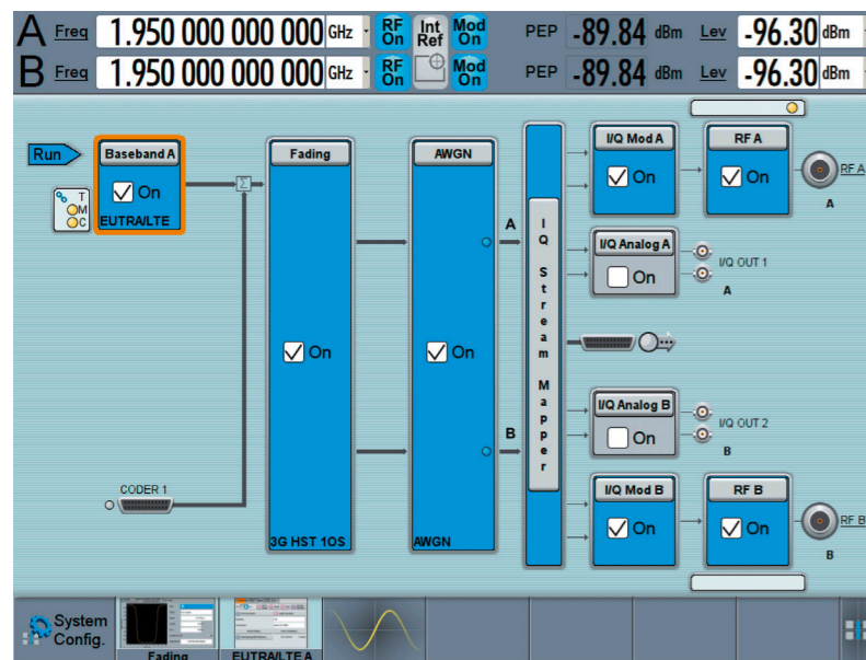
The R&S®SMW200A is perfect for LTE base station performance tests in line with 3GPP TS36.141. In this example, the block diagram (screenshot on the left) and fading settings (screenshot below) for testing with high-speed train fading are shown.
