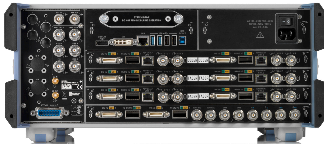
Rear panel of the R&S®SMW200A.
