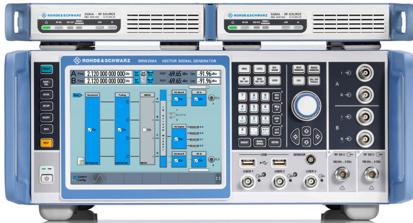
R&S®SMW200A vector signal generator with two R&S®SGMA signal generator modules on top
