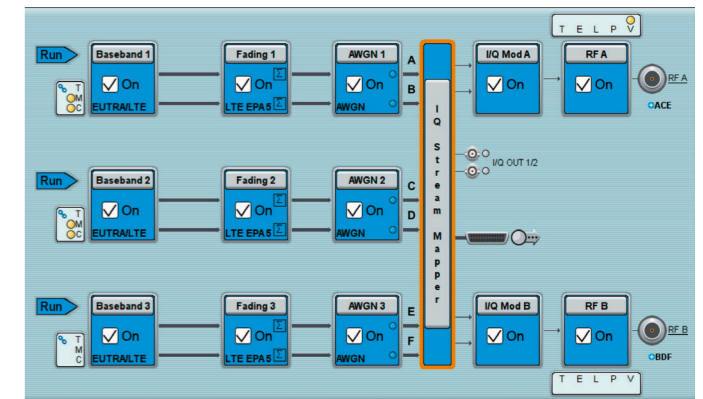
Block diagram of the R&S®SMW200A configured for the generation of an LTE Release 11 fciCIC test scenario. One R&S®SMW200A simultaneously generates the LTE serving cell as well as the two aggressor cells, each with 2x2 MIMO, with correlated fading channels.
