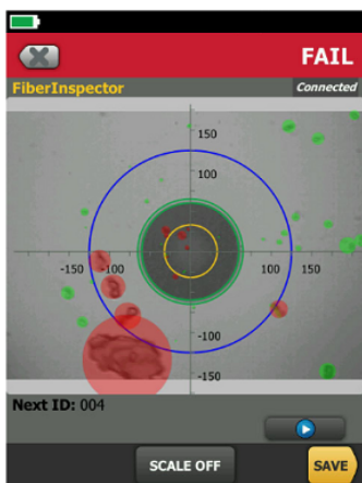
FiberInspector probe
