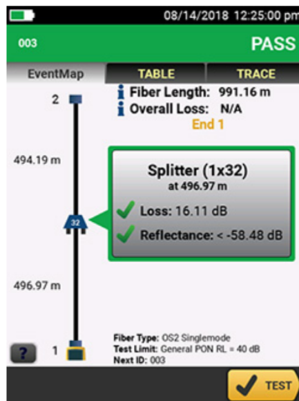
Splitter as seen on an EventMap
