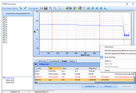
Setting span event parameters using LinkWare PC
