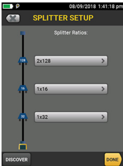
Splitter setup
