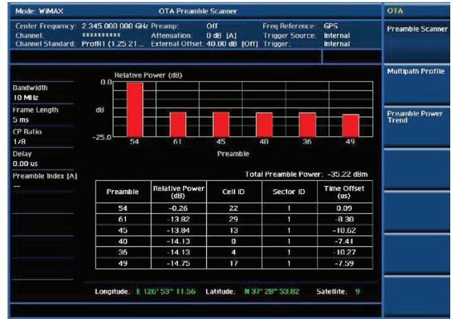
WiMAX OTA preamble scanner
