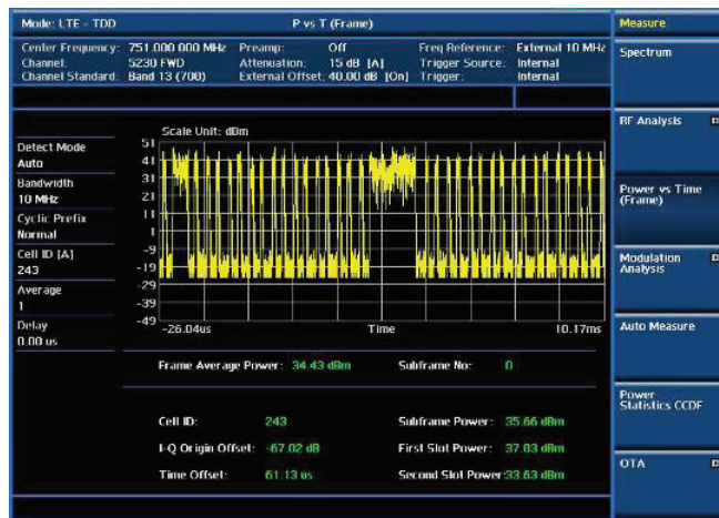
LTE power vs. time (frame)
