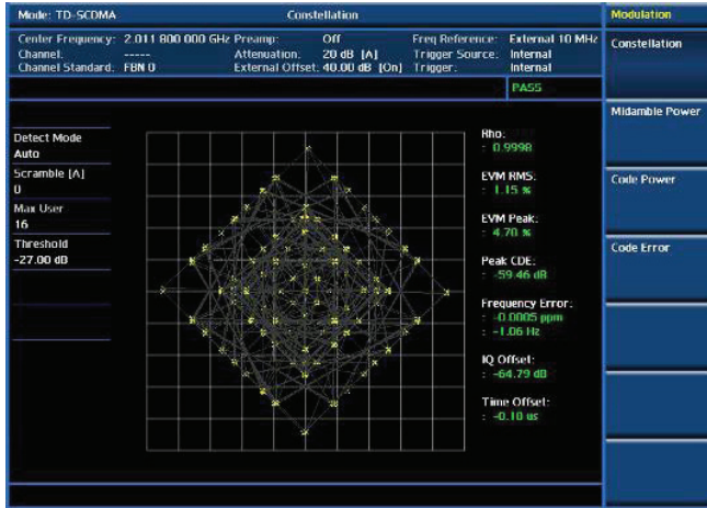
TD-SCDMA constellation
