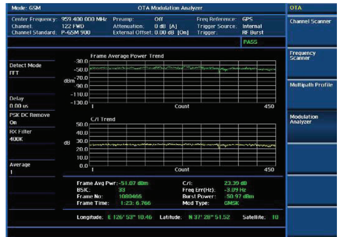
GSM OTA modulation analyzer
