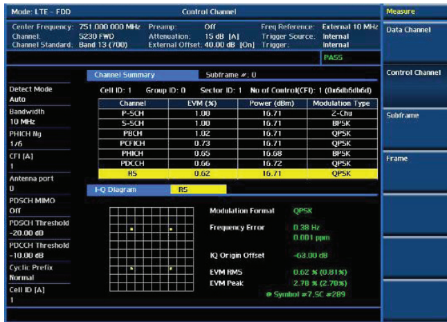
LTE control channel summary
