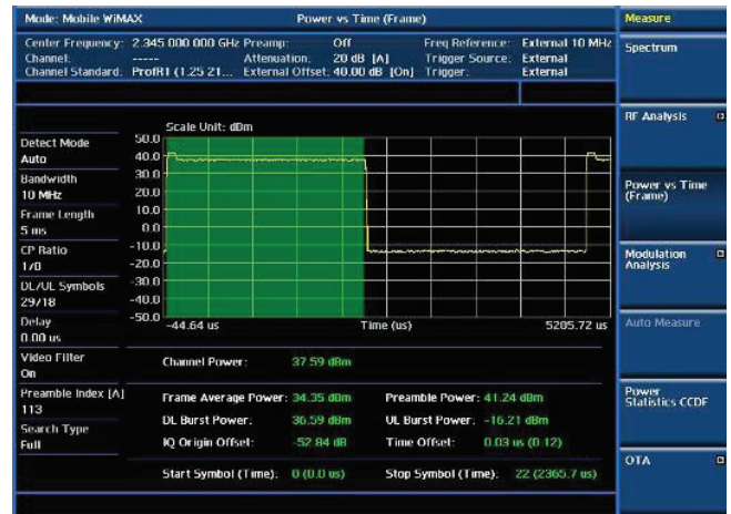
WiMAX Power vs. time (frame)
