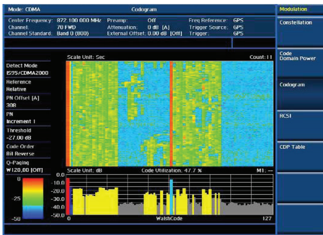
CDMA codogram
