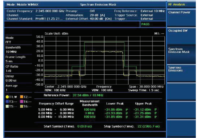
WiMAX spectrum emission mask
