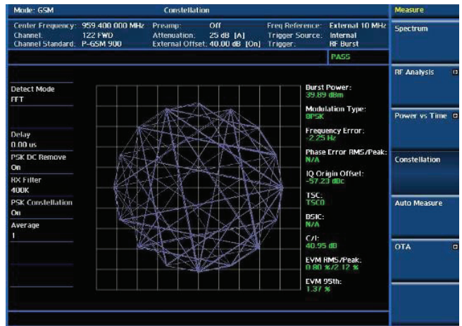
GSM constellation
