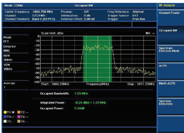
CDMA occupied bandwidth
