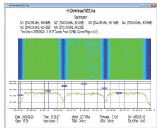
JDViewer spectrogram, RSSI
