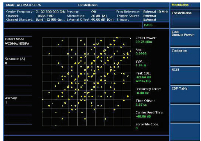
WCDMA constellation
