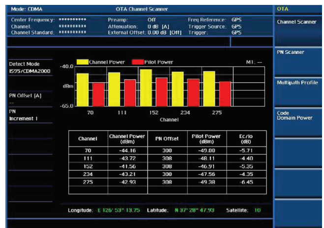
CDMA OTA channel scanner
