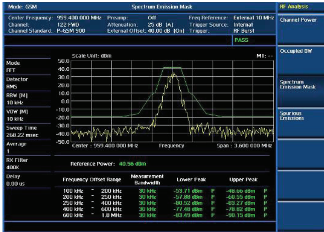
GSM spectrum emission mask
