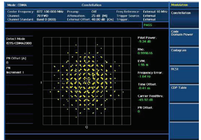
CDMA constellation
