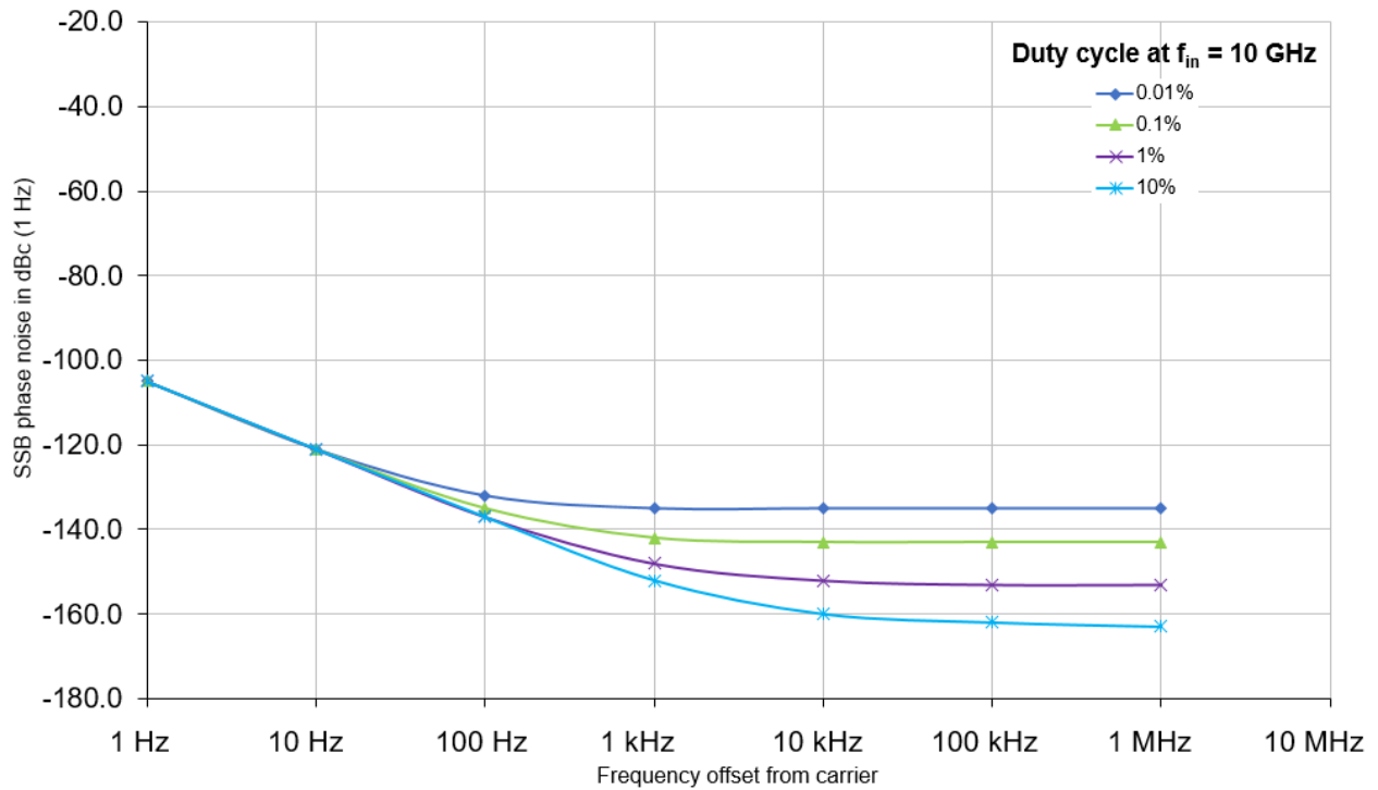
Typical AM noise sensitivity at f_{in} = 10 GHz (start offset = 1 Hz, correlation factor = 1, signal level = 10 dBm, gating = on)
