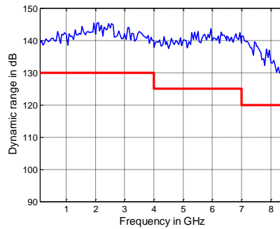
Dynamic range in dB versus frequency for the R&amp;S®ZNB8.
