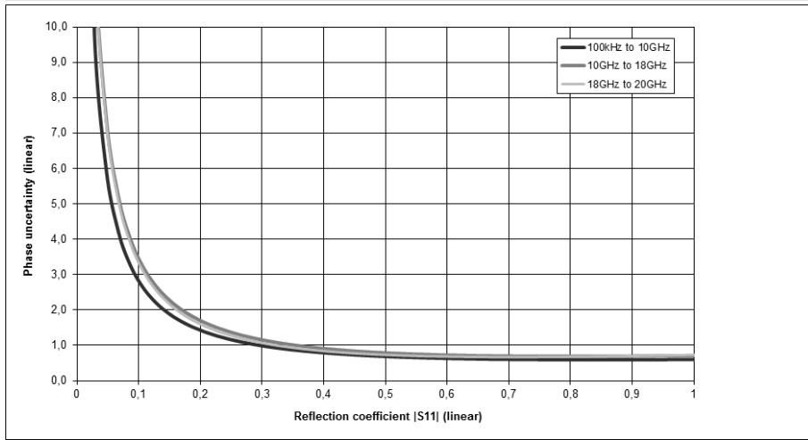
Typical accuracy of reflection magnitude and reflection phase measurements for the R&S® ZNBT20 in the frequency range from 100 kHz to 20 GHz, calibrated with a R&S® ZV-Z235 calibration kit that has been characterized with a DAkkS-accredited calibration. Analysis conditions: S_{12} = S_{21} = 0 , cal. power -10 dBm, meas. power -10 dBm.
