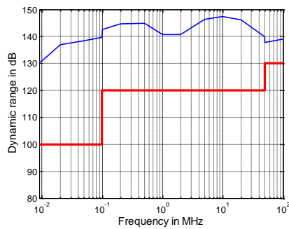
Dynamic range in dB versus frequency for the R&amp;S®ZNB8.
