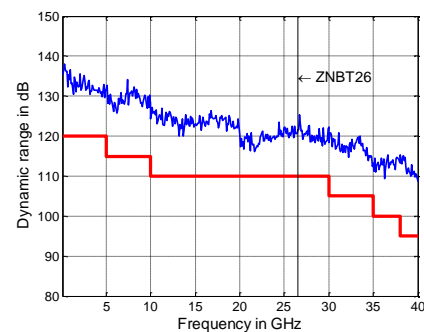
Dynamic range in dB versus frequency for the R&amp;S®ZNB26/40.
