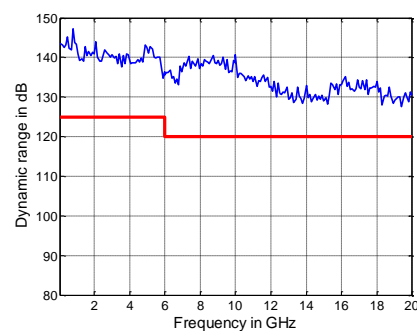
Dynamic range in dB versus frequency for the R&amp;S®ZNB20.
