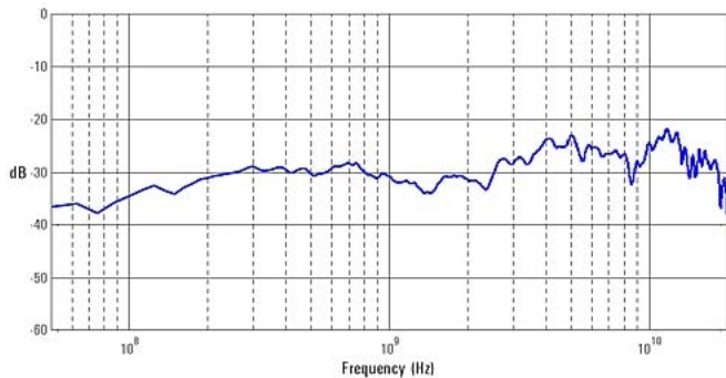
Common mode rejection ratio of 1169B
