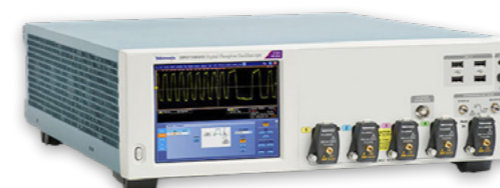
Tektronix DPS75004SX | ATI Performance Oscilloscope System, 33/50 GHz
