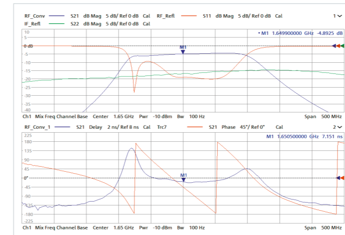
Results of a converter measurement including return loss, conversion loss, phase and group delay
