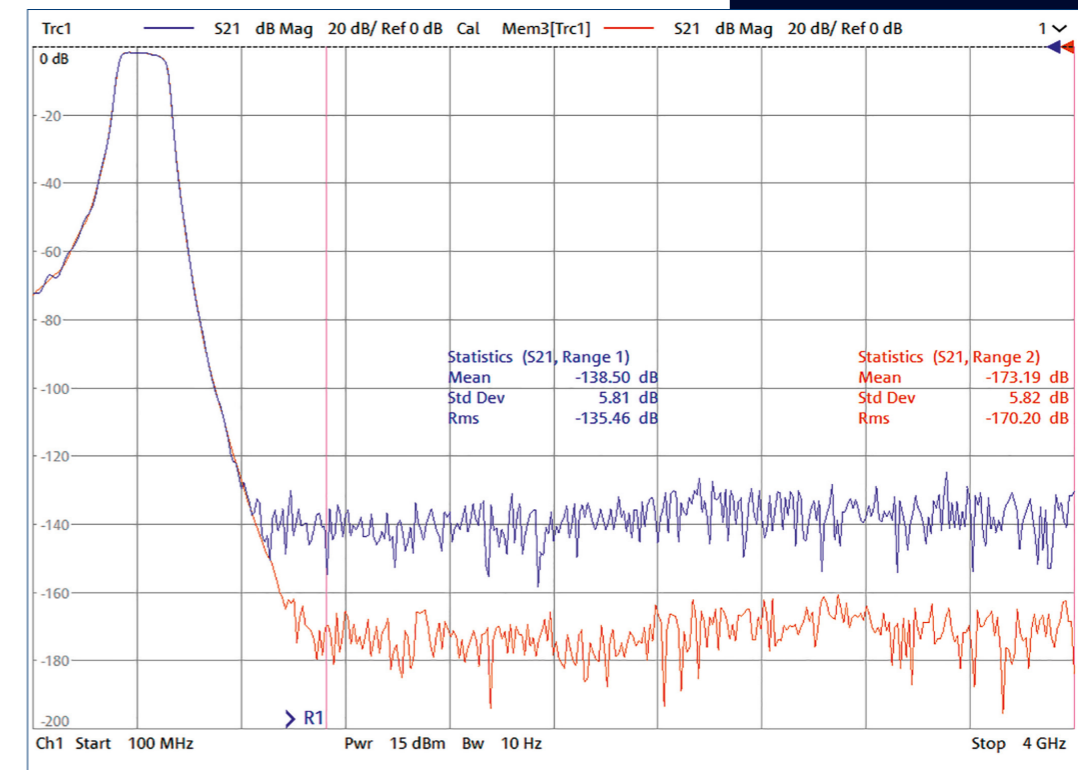
Dynamic range: at maximum specified output power, without options (blue trace: at 10 Hz IF bandwidth); at maximum specified output power, in reversed coupler mode, with receiver step attenuator set to 0 dB (red trace: at 1 Hz IF bandwidth)
