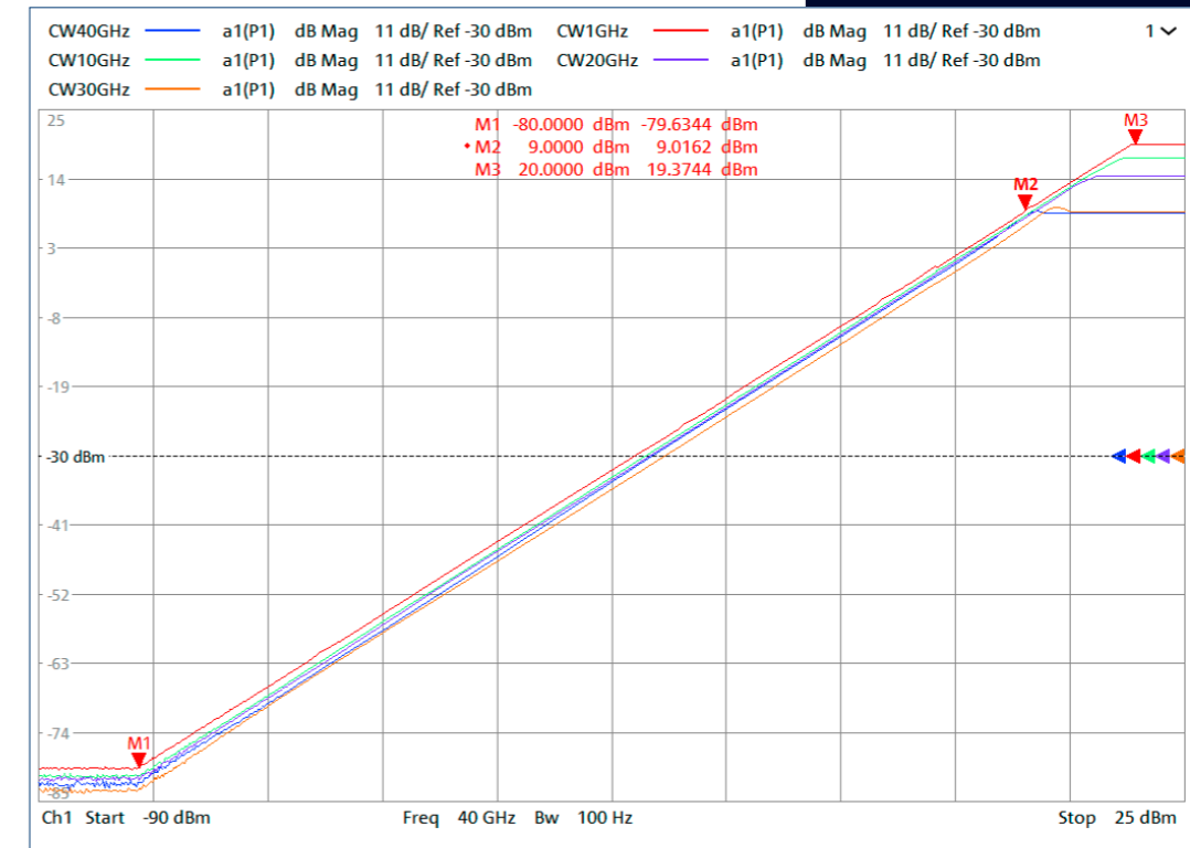
Maximum power sweep range of up to 100 dB
