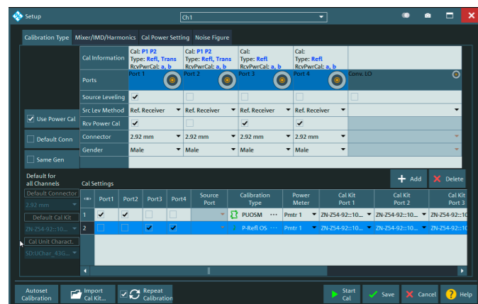
The R&S®SMARTerCal merges system error correction, receiver power calibration and absolute source level calibration.
