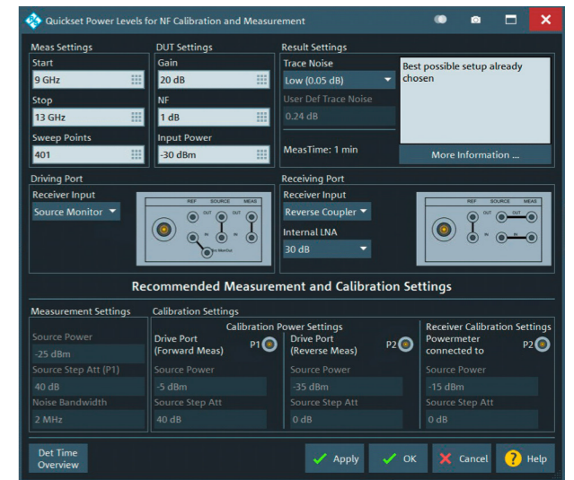
Quickset dialog for interactive and semi-automatic configuration of optimal test parameters and R&S®ZNA hardware
