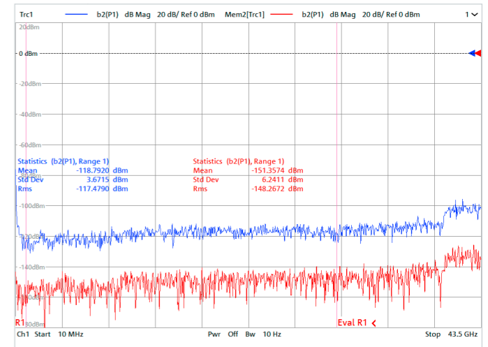
The sensitivity of the R&S®ZNA26/R&S®ZNA43 receivers can reach –150 dBm (lower frequency end, typical, at 1 Hz IFBW, direct channel access/reversed coupler, receiver step attenuator in 0 dB position). The sensitivity of the b1 and b2 receivers is increased further by using the R&S®ZNAxx-B302 and R&S®ZNAxx-B501 preamplifiers.
