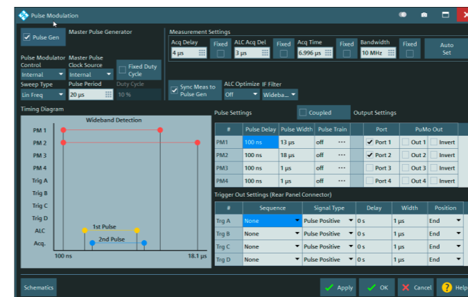
The configuration of ALC supported measurements under pulsed condition allows detailed settings to match ALC and pulse parameters. For instance, to allow short pulses, ALC control and measurement can be set to successive pulses.
