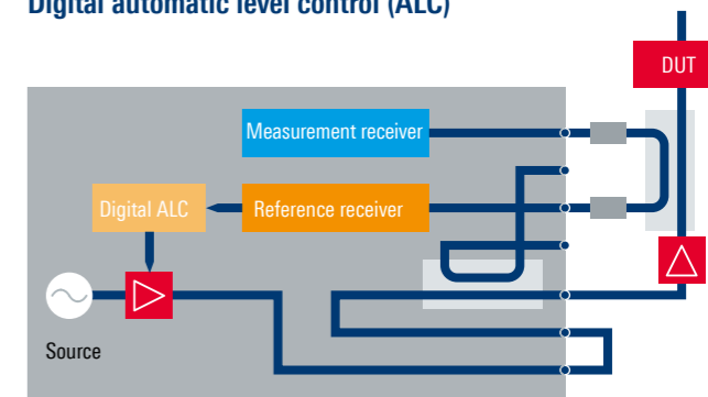
ALC operation: in a high-power setup with an external preamplifier and a directional coupler, the source power is controlled to match the preamplifier output power. This compensates for drift effects, making the output power very precise and stable.
