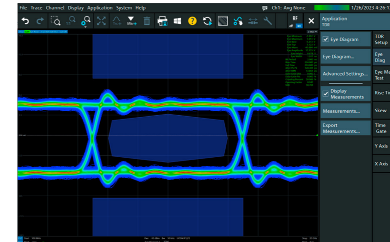
Eye diagram mask test with synthetic signal predistortion
