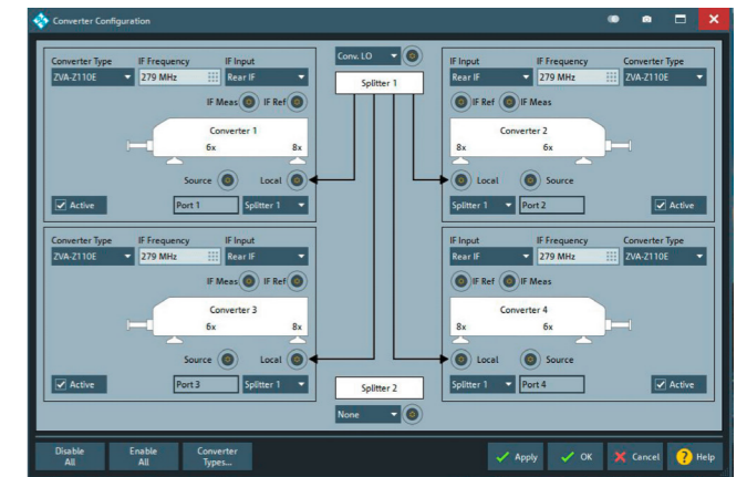
Software configuration
