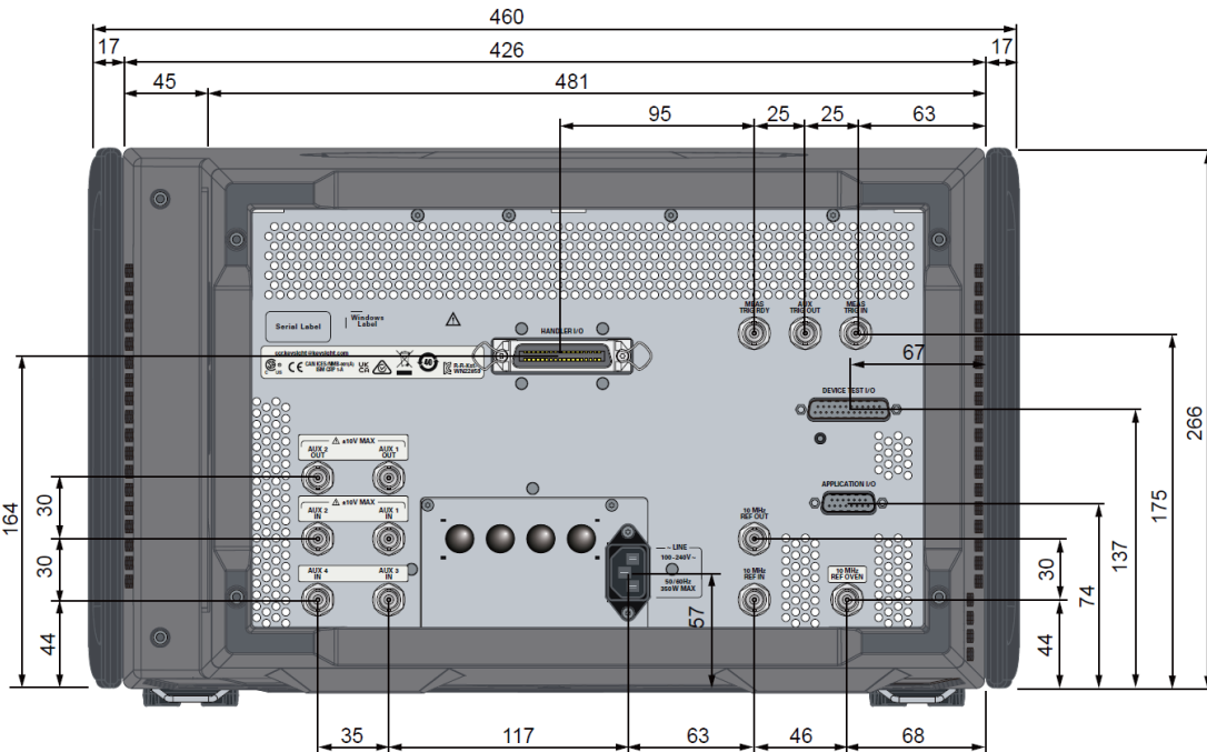
Dimensions (rear view, E5081A with option 1E5/175, in millimeters)
