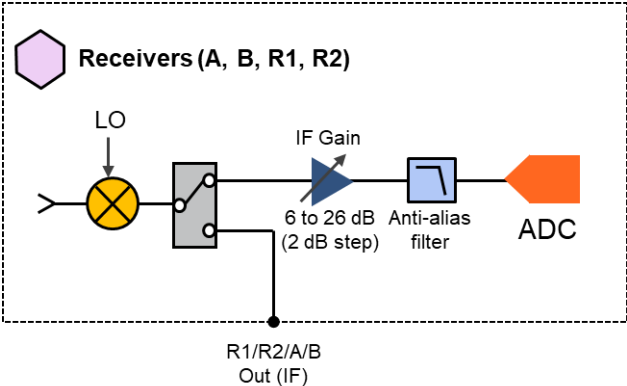
Receiver block diagram (port 1 and 2)
