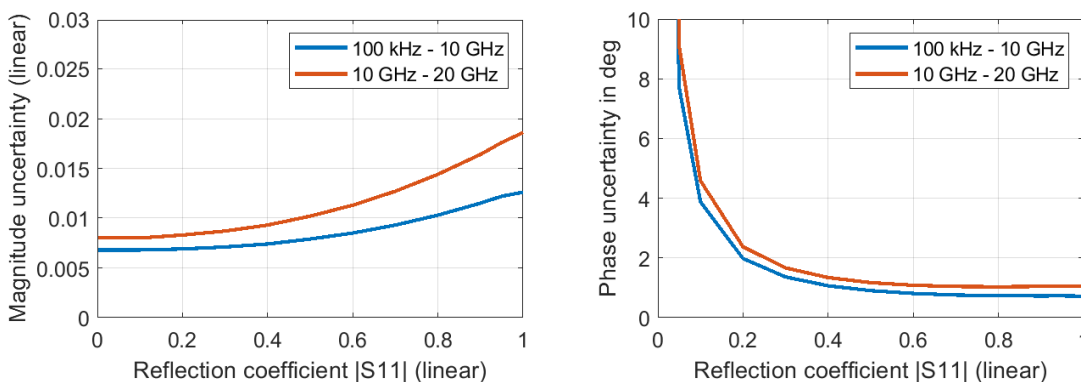
Typical uncertainty of reflection magnitude and reflection phase measurements for the R&S®ZNB20 in the frequency range from 100 kHz to 20 GHz; analysis conditions: S_{12} = S_{21} = 0 , cal. power: -10 dBm, meas. power: -10 dBm
