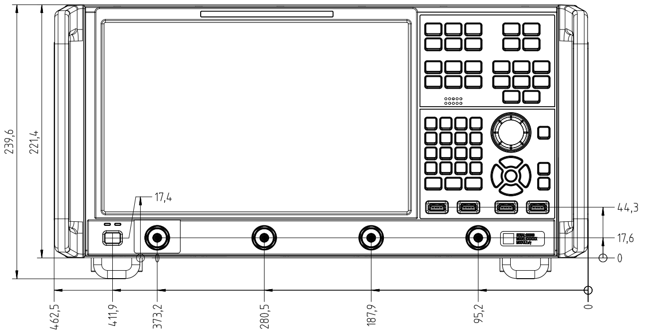
Front view of the R&S®ZNB
