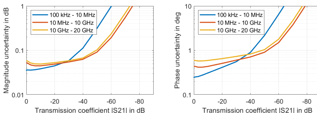
Typical uncertainty of transmission magnitude and transmission phase measurements for the R&S®ZNB20 in the frequency range from 100 kHz to 20 GHz; analysis conditions: S_{11} = S_{22} = 0 , cal. power: -10 dBm, meas. power: -10 dBm
