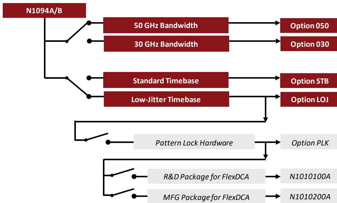
Figure 27. N1094A/B configuration chart
