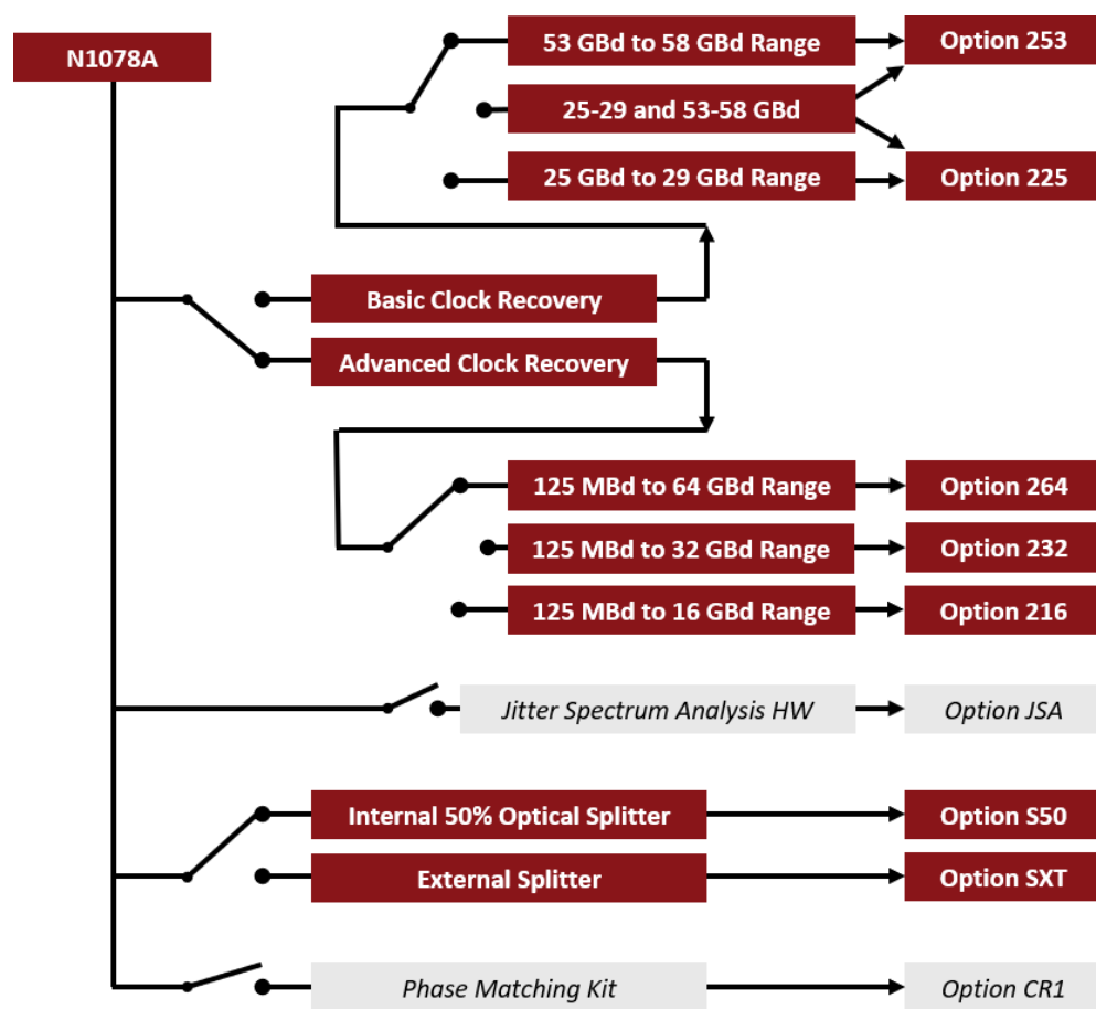
Figure 20. N1078A Single-mode optical/electrical clock recovery with options 264 and S50
