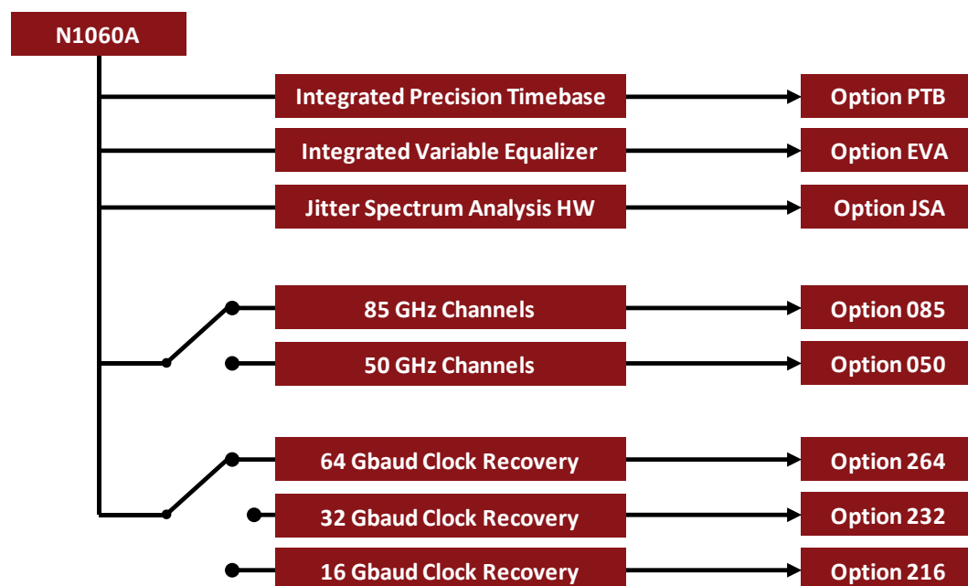
Figure 15. N1060A configuration chart
