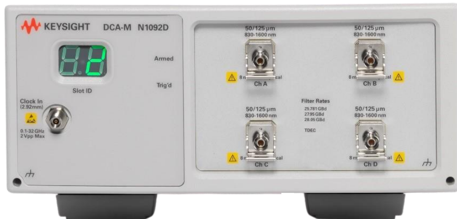
Figure 24. N1092D quad optical DCA-M with options 30A, 280 and 168
