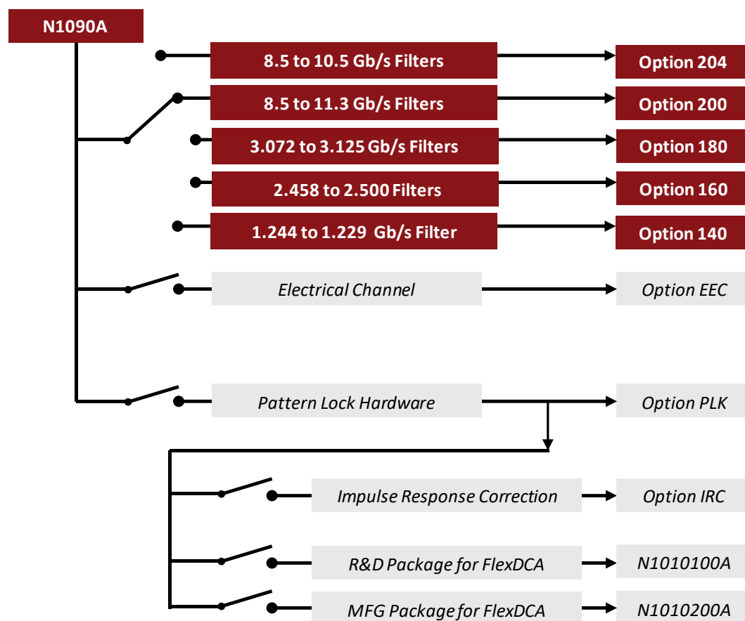
Figure 23. N1090A configuration chart
