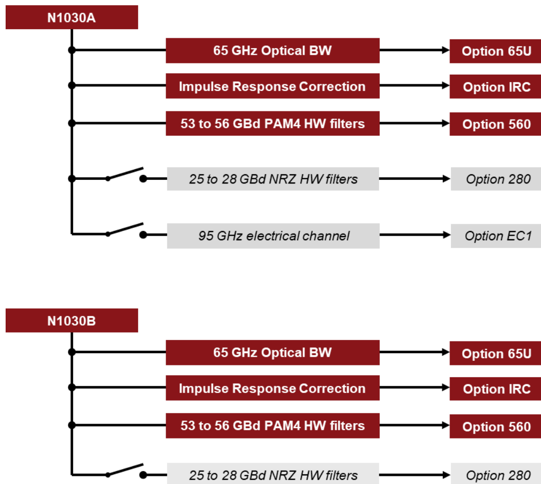
Figure 5. N1030A/B configuration chart
