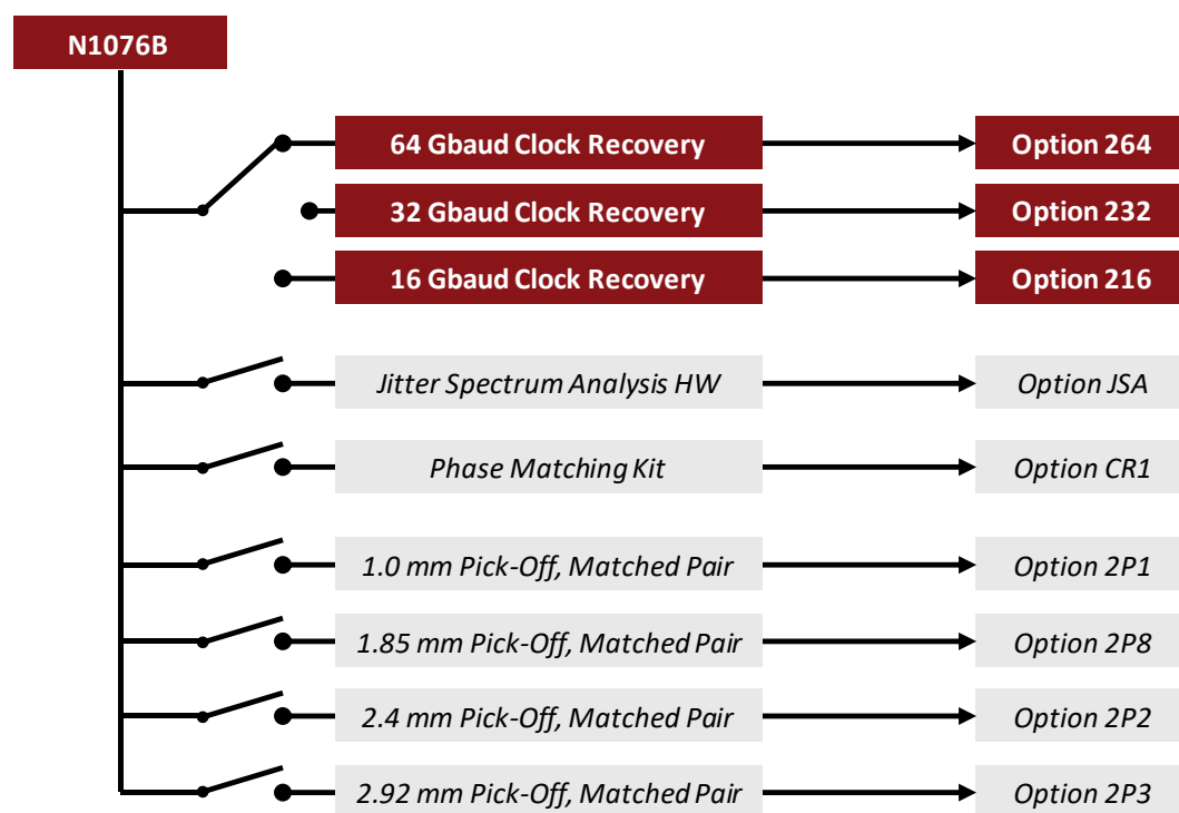
Figure 16. N1076B Electrical clock recovery with option 264
