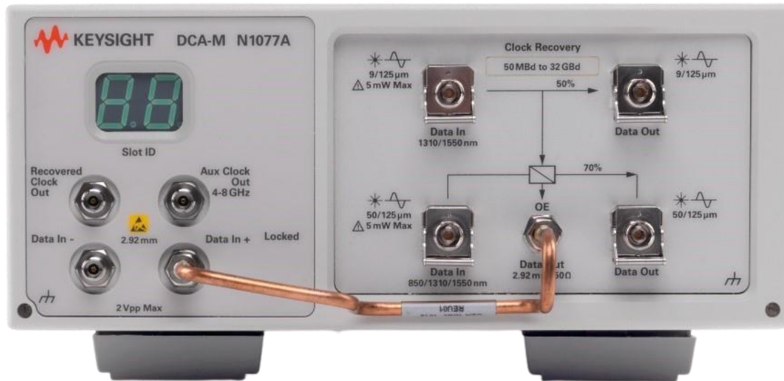
Figure 18 N1077A Single- & multimode optical/electrical clock recovery with options 232 and SMS
