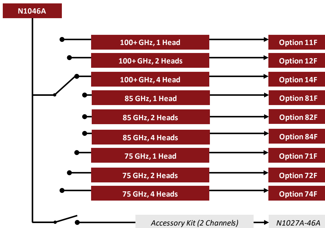
Figure 11. N1046A configuration chart
