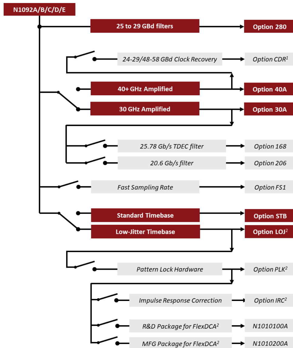
Figure 25. N1092A/B/C/D/E configuration chart
