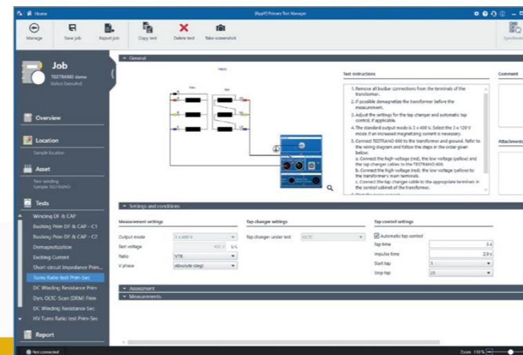
PTM supports you in the best possible way during execution of diagnostic tests via wiring diagrams and asset-specific test plans according to international standards.
