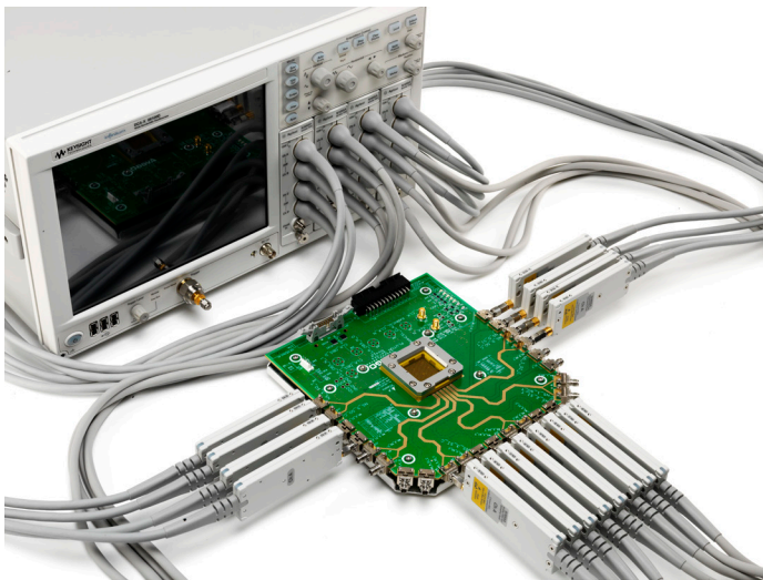
2- to 16-channel TDR/TDT/S-parameter measurement system.
