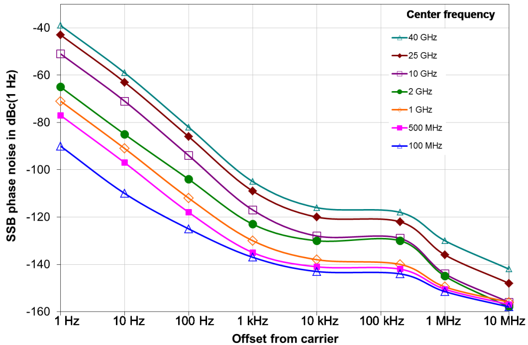
Typical phase noise at different center frequencies (with the R&S®ESW-B4 option for offsets ≤ 10 Hz).
