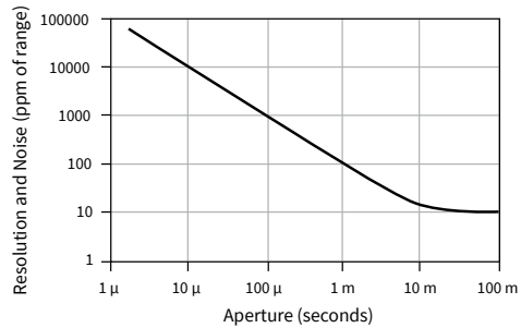
Figure 1. Noise and Resolution versus Measurement Aperture, Typical
