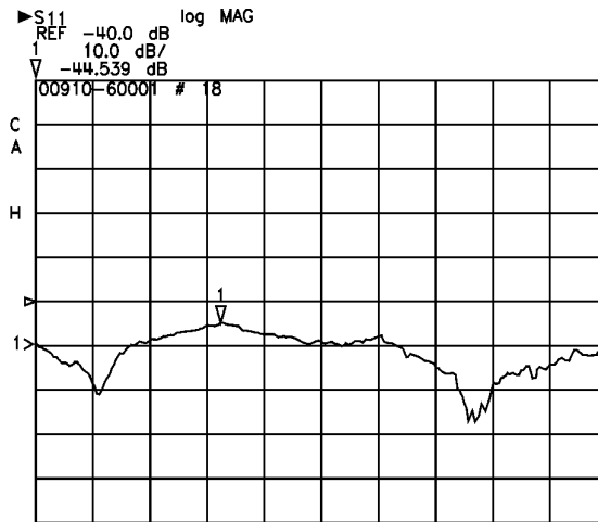
Typical Termination Return Loss
