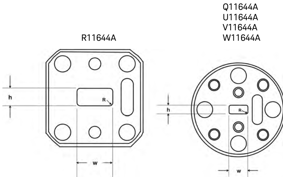
Figure 2-1 \frac{1}{4} Wavelength Shims
