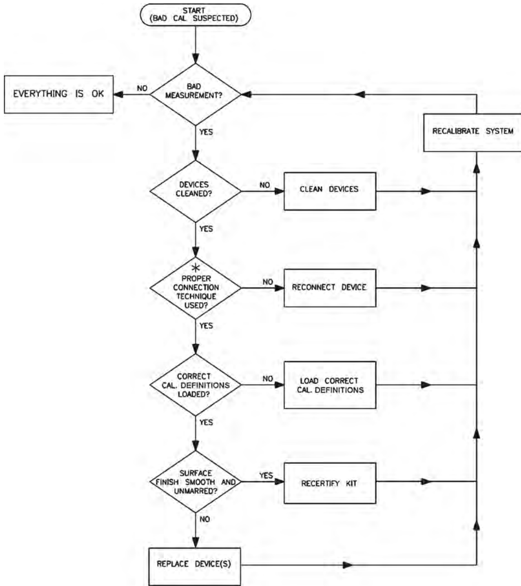
Figure 6-1 Troubleshooting Flowchart
