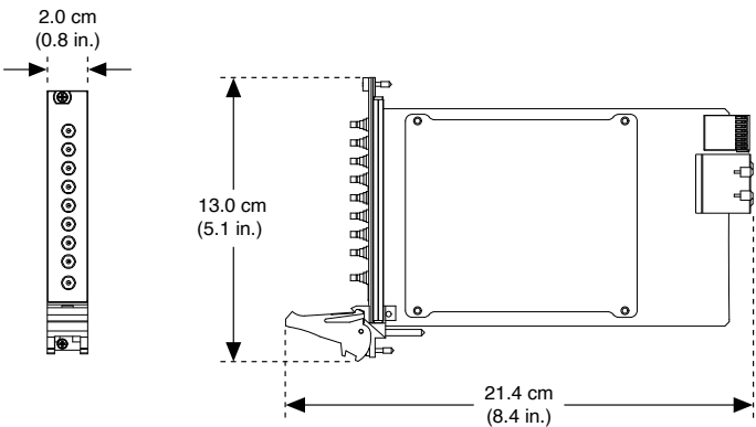
Figure 1. PXIe-5105
