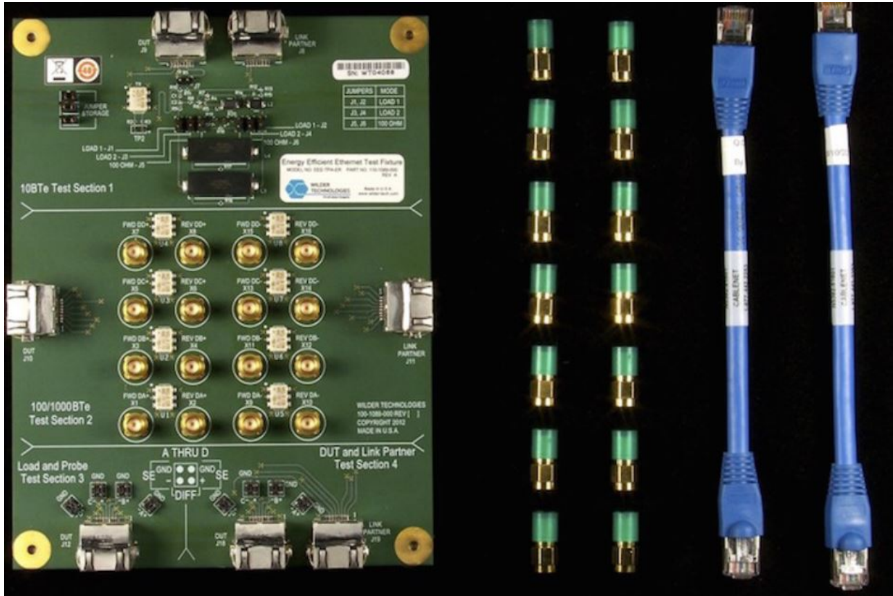
Figure 8. The EEE-TPA-ERK Wilder Technologies Energy Efficient Ethernet test fixture allows you to test to the 10BASE-Te, 100BASE-TXe and 1000BASE-Te Energy Efficient Ethernet standards. Sold separately through Wilder-Technologies.
