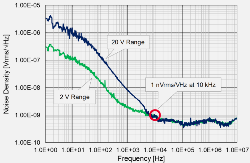
Figure 6. HC-ULNF and ULNF provide excellent noise density performance
