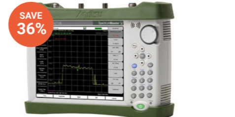
Anritsu Spectrum Analyzers-Hand Held MS2712E Spectrum Master, 9 kHz - 4 GHz Spectrum Analyzer BUY USED FROM: £12,656 € 14,223
