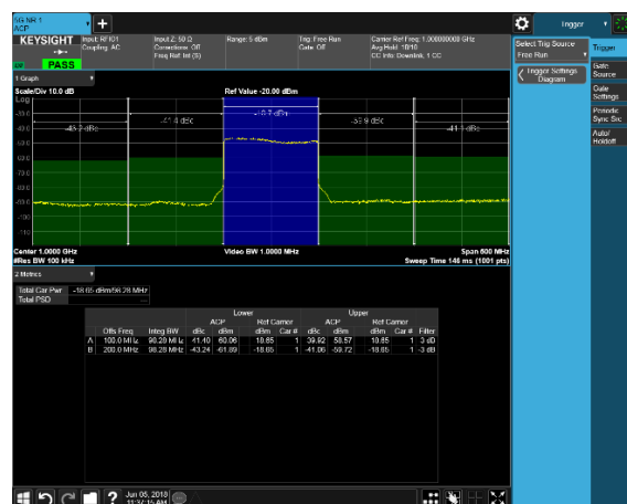
Figure 2. 5G NR adjacent channel power (ACP) results
