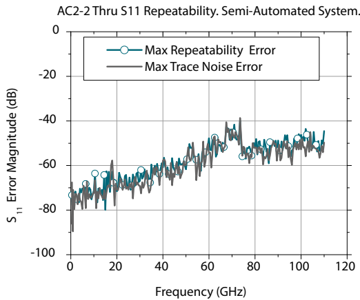
The maximal probe contact repeatability error of the calibrate S 11 -parameter of the AC2-2 thru standard by T110 probes. Semi-automated system. Ten contact circles.
