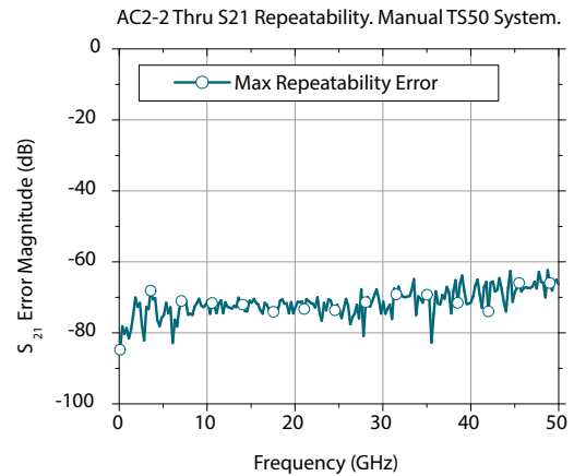
The maximal probe contact repeatability error of the calibrate S 21 -parameter of the AC2-2 thru standard by T50 probes. Manual probe system TS50.
