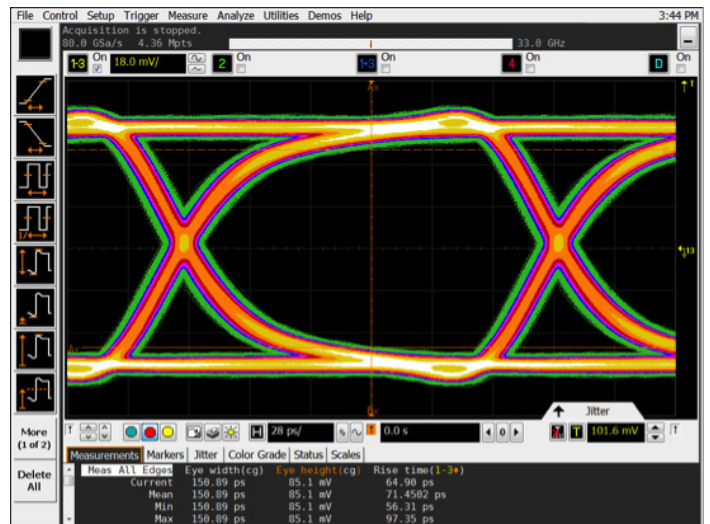
Figure 2. Signal through N7010A active termination adapter; N7010A does not inherently contribute noise
