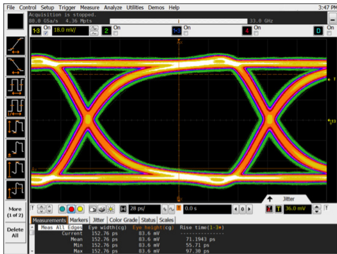
Figure 1. Direct signal connect to Infiniium scope
