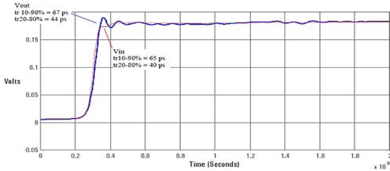
Graph of Vin and Vout of 1169A and N5381B solder-in head with a 25 \Omega 58 psec step generator
