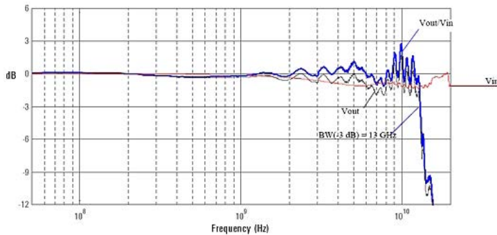
Frequency response of 1169A and N5381B with a 25 \Omega source
