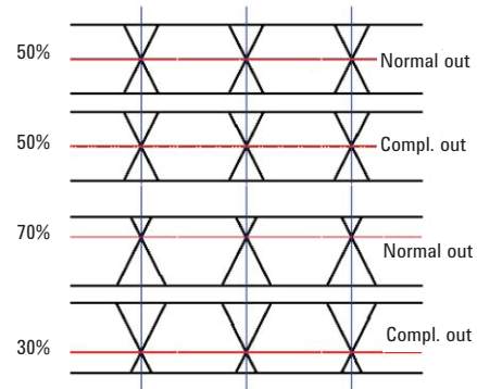
Figure 1. Variable crossover
