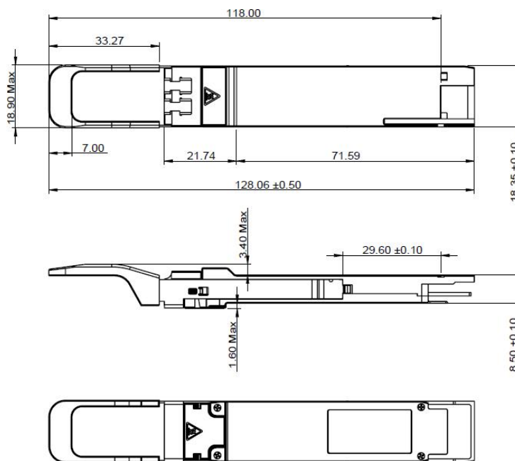
Figure 5. Mechanical Outline
