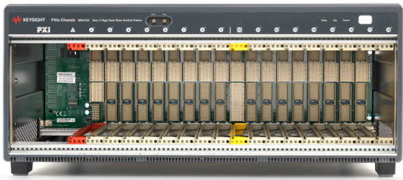
Figure 1. M9018B and M9019A 18-slot PXIe Gen 3 chassis
