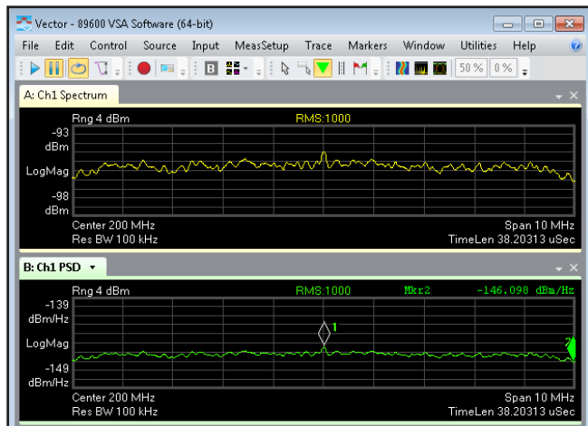
Figure 4. Noise power spectral density (NSD) measured with the 89600 VSA software on one channel of the M9703A. With a very low NSD down to -146 dBm/Hz, the M9703A has comparable performance to some 16-bit digitizers.
