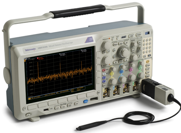
The optional TPA-N-VPI adapter enables any active, 50 Ω TekVPI probe to be connected to the RF input.
