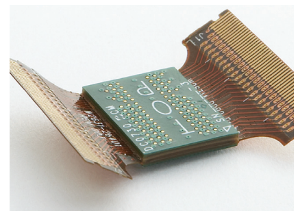
Figure 14. DDR2 BGA probe adapter for oscilloscopes and logic analyzers.
