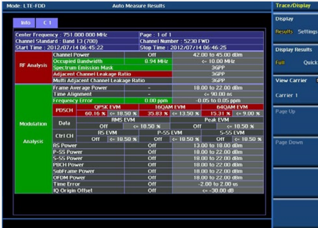
RF and Modulation analysis — Auto Measure
