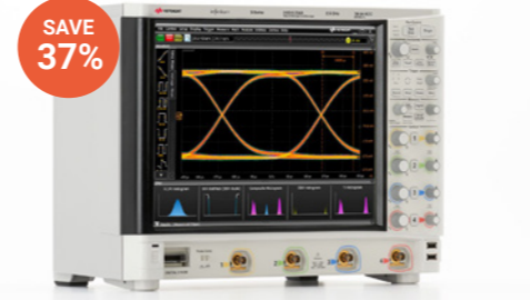
SAVE 37% Keysight Technologies Oscilloscopes DSOS254A >3GHz-<8GHz Oscilloscope - Infiniium S Series 2.5 GHz 4 channel; Memory - 400Mpts/ch memory installed BUY USED FROM: £24,521 € 27,558
