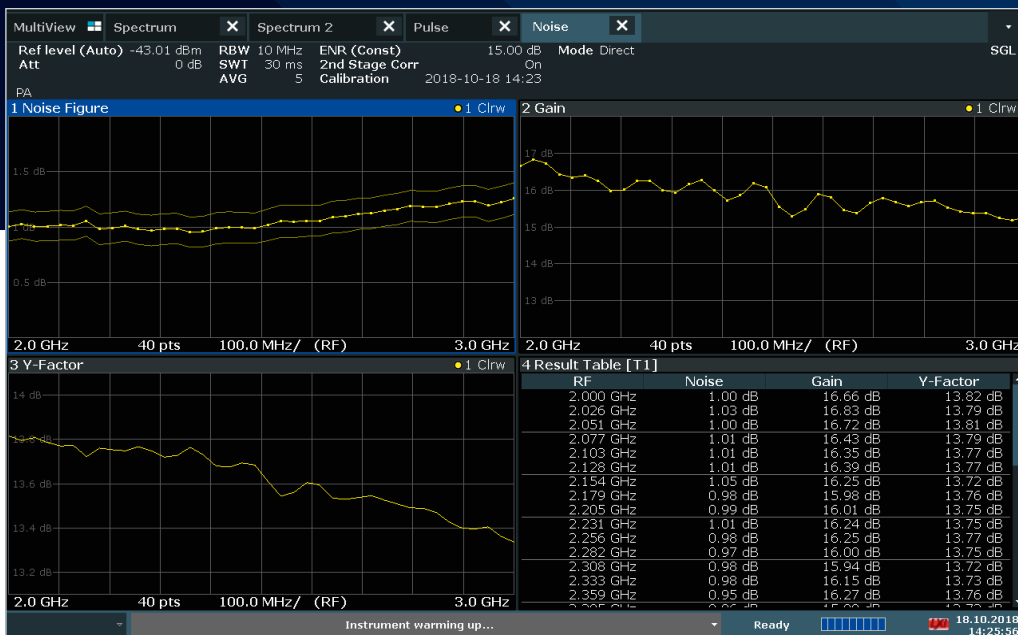
Fig. 1: Noise figure and gain measurement with R&S®FSx-K30 application firmware. In addition to the result table, the noise figure traces and the calculated gain, the Y factor can also be displayed.
