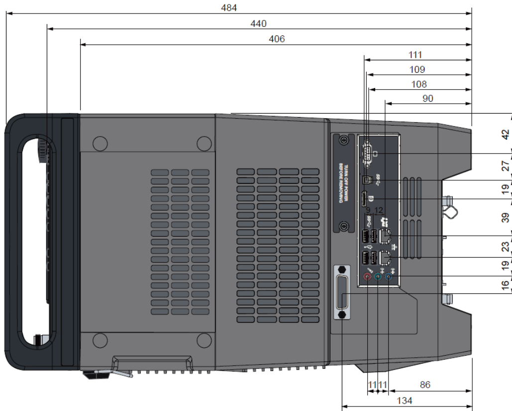
Figure 9. Side view (mm)
