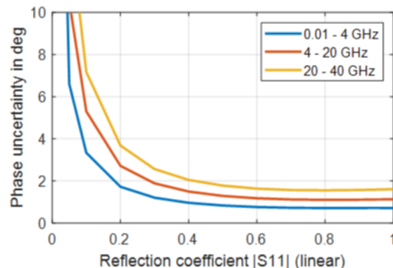
Uncertainty of reflection magnitude and reflection phase measurements for the R&S®ZNB40 model .72 in the frequency range from 10 MHz to 40 GHz; analysis conditions: S_{12} = S_{21} = 0 , cal. power -10 dBm, meas. power -10 dBm
