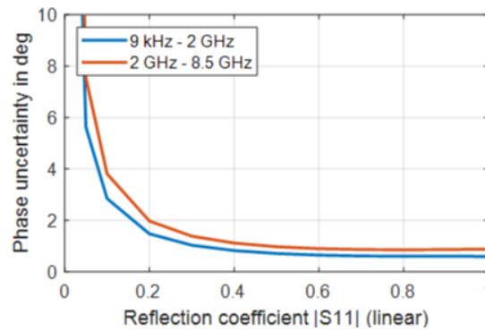
Uncertainty of reflection magnitude and reflection phase measurements for the R&S®ZNB4 in the frequency range from 9 kHz to 4.5 GHz, for the R&S®ZNB8 in the frequency range from 9 kHz to 8.5 GHz; analysis conditions: S_{12} = S_{21} = 0 , cal. power -10 dBm, meas. power -10 dBm
