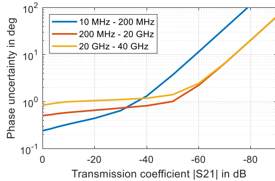
Uncertainty of transmission magnitude and transmission phase measurements for the R&S®ZNB40 model .72 in the frequency range from 10 MHz to 40 GHz; analysis conditions: S_{11} = S_{22} = 0 , cal. power -10 dBm, meas. power -10 dBm
