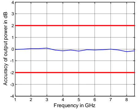
Output power accuracy in dB versus frequency for the R&S ZNB8
