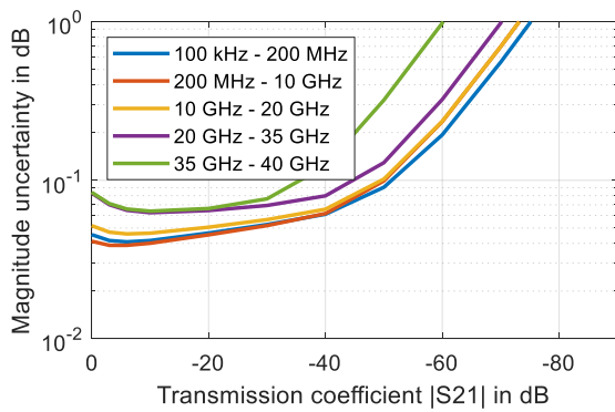
Uncertainty of transmission magnitude and transmission phase measurements for the R&S®ZNB40 model .82 and .84 in the frequency range from 100 kHz to 40 GHz; analysis conditions: S_{11} = S_{22} = 0 , cal. power -10 dBm, meas. power -10 dBm
