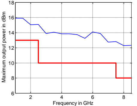
Maximum output power in dBm versus frequency for the R&S ZNB8
