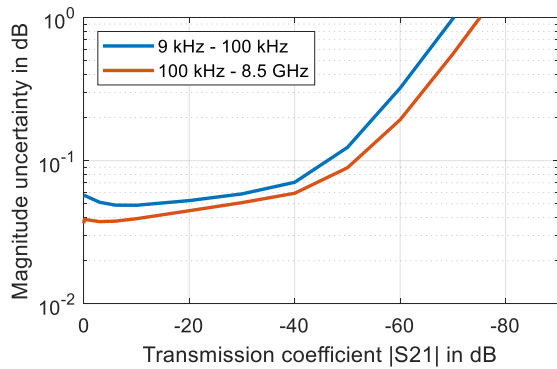
Uncertainty of transmission magnitude and transmission phase measurements for the R&S®ZNB4 in the frequency range from 9 kHz to 4.5 GHz, for the R&S®ZNB8 in the frequency range from 9 kHz to 8.5 GHz; analysis conditions: S_{11} = S_{22} = 0 , cal. power -10 dBm, meas. power -10 dBm
