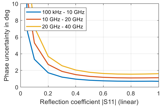
Uncertainty of reflection magnitude and reflection phase measurements for the R&S®ZNB40 model .82 and .84 in the frequency range from 100 kHz to 40 GHz; analysis conditions: S_{12} = S_{21} = 0 , cal. power -10 dBm, meas. power -10 dBm
