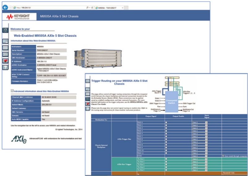
Figure 3. Chassis web page
