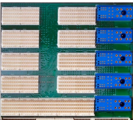
Figure 1. 5-slot AXIe backplane
