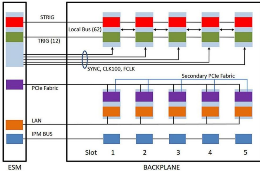
Figure 2. M9505A backplane block
