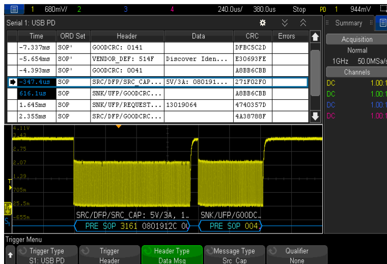
Figure 14. USB PD decode on an InfiniiVision X-Series
